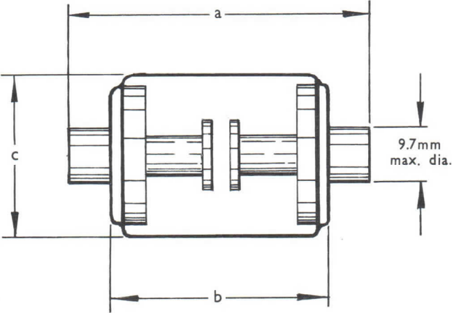
Outline B
