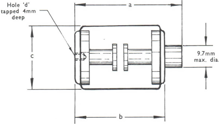
Outline A
