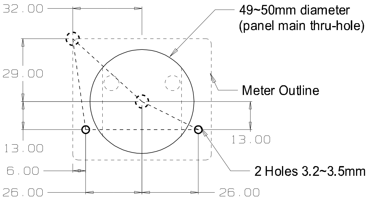
Model 85 Meter Cutout
