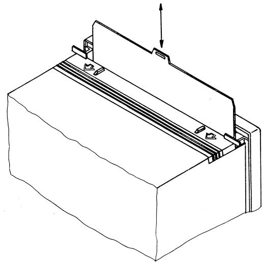
Picture 8a: Exchanging of scales
