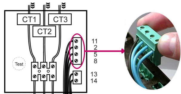
Picture 14: Connections for full equipped device, position of battery and picture of connectors
