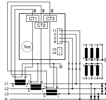
Picture 13: Three phase system (four wire unbalanced - 4u)
