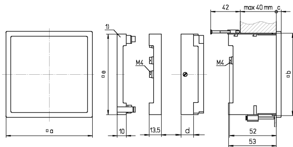
Picture 15: Dimensional drawing EQXX07 and YQXX07 (all dimensions are in mm)
