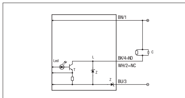
NPN – NO + NC
