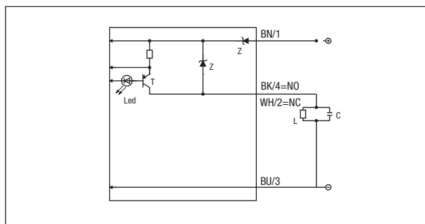
PNP – NO + NC
