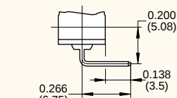
PCB Terminals LH Side with Location Pins 0.024 x 0.020 (0.6 x 0.5)
