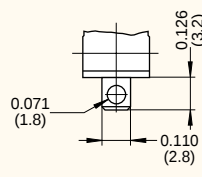
PCB Terminals RH Side w/o Location Pins 0.024 x 0.020 (0.6 x 0.5)
