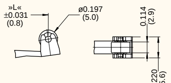
Simulated Roller - Plastic
