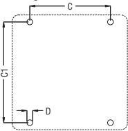
Drilling for enclosure fixing
