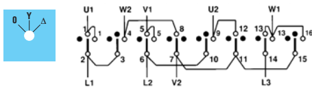
12 - Star-delta switch
