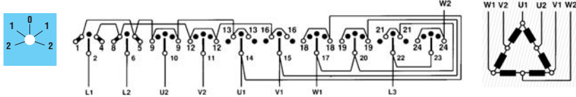
20 - Pole-changing switch with reversing (Dahlander)
