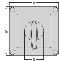
Mounting in enclosure
