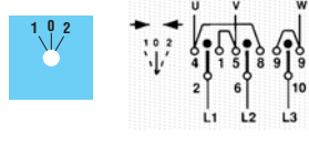
26 - Reversing switch, spring return to 0
