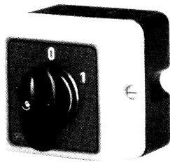
ON-OFF 3 Pole, 10 Amp. M 10 PA 3
