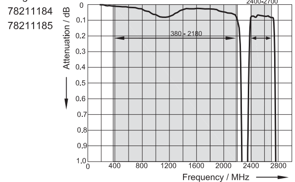
Diagram 2 Port 1 ↔ Port 3 Port 2 ↔ Port 3
