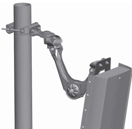
Off-set Downtilt
