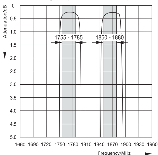
Diagram III (Port 2 ↔ Port 3 / Port 5 ↔ 6)
