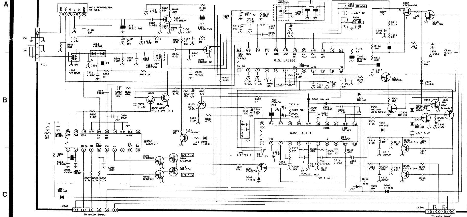
TUNER BOARD PW 2074-1
