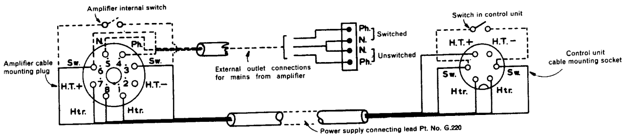
Fig. 3. EXTERNAL SUPPLY CONNECTION ARRANGEMENTS FOR SC2 CONTROL UNIT
