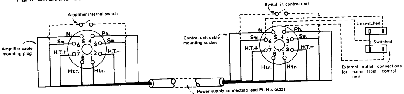
Fig. 4. EXTERNAL SUPPLY CONNECTION ARRANGEMENTS FOR SC22 CONTROL UNIT
