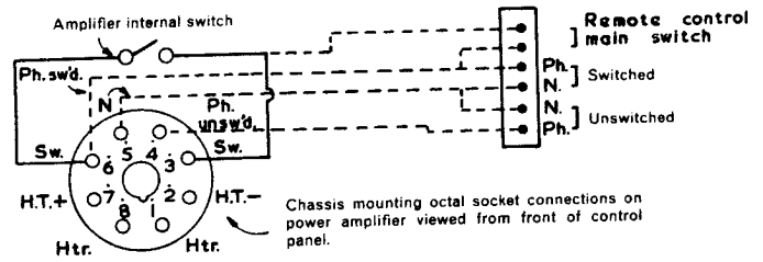
Fig. 2. BASIC CONNECTIONS OF EXTERNAL POWER SOCKET
