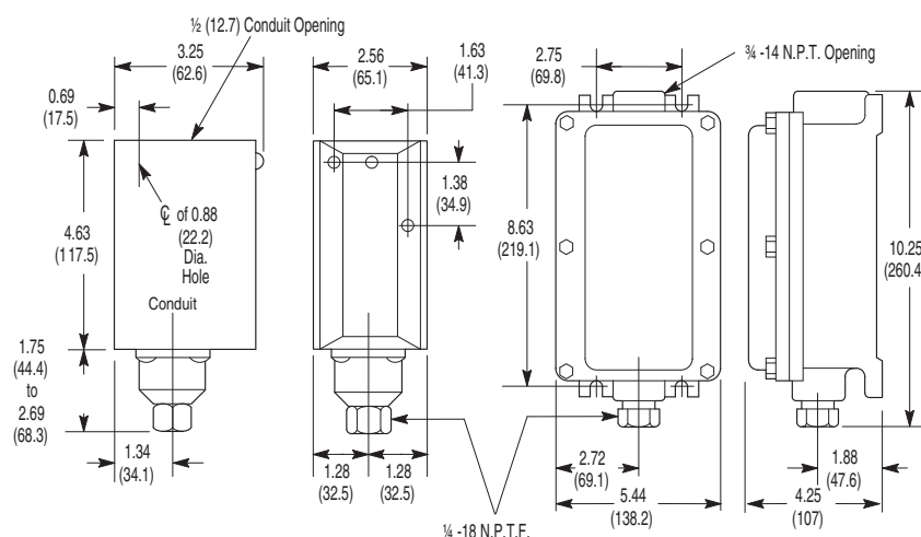
Type 1 Approximate Shipping Weight 2.0 (.9 kg)
