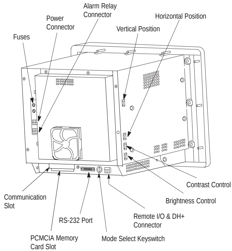
PanelView 1400e Rear View
