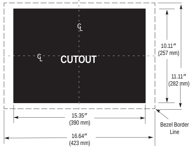
Panel Cutout for PanelView 1000e Clip Mount Keypad Terminal
