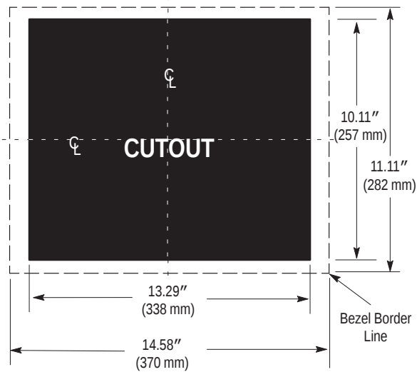
Panel Cutout for PanelView 1000e Clip Mount Touch Screen Terminal
