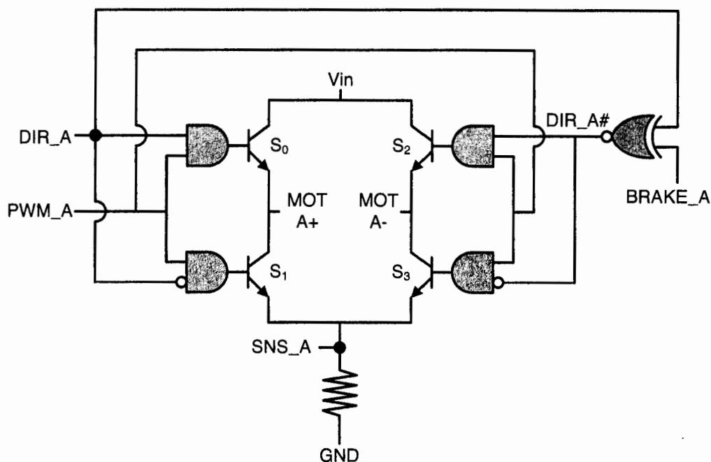
Figure 9.6 H bridge connections
