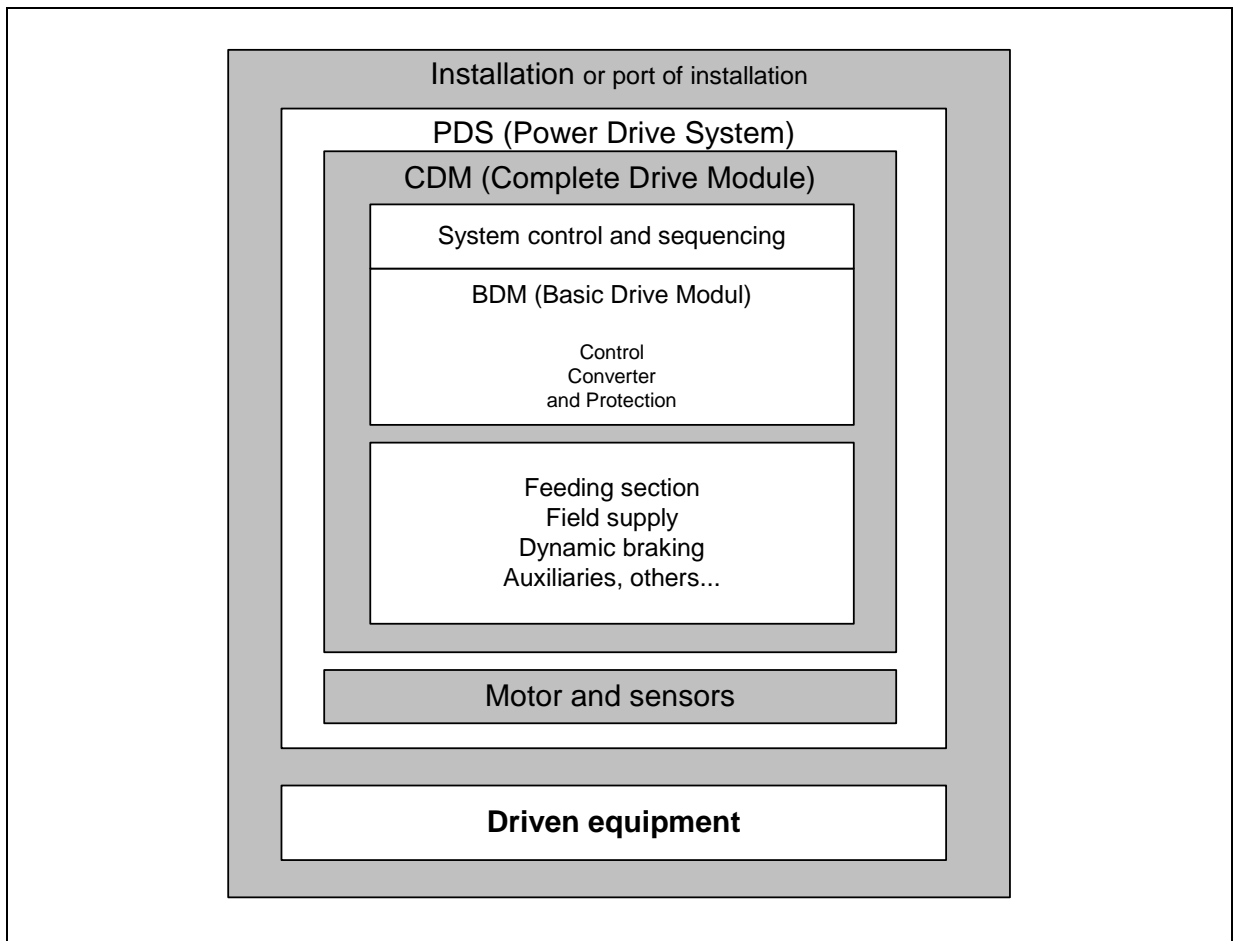
Fig. 2-3 Power Drive System (PDS) according to EN 61800-3
