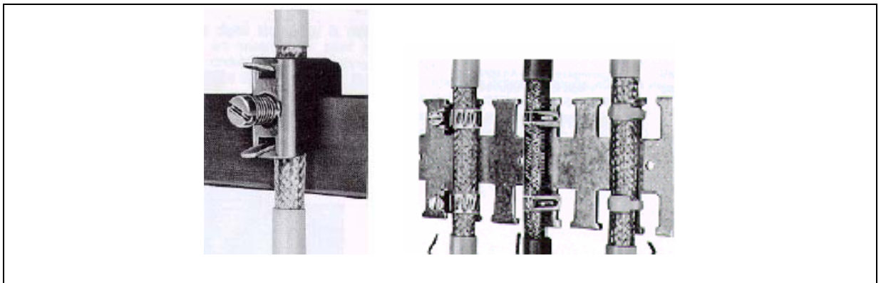
Fig. 4-8 Examples for connecting shields to a shield rail
