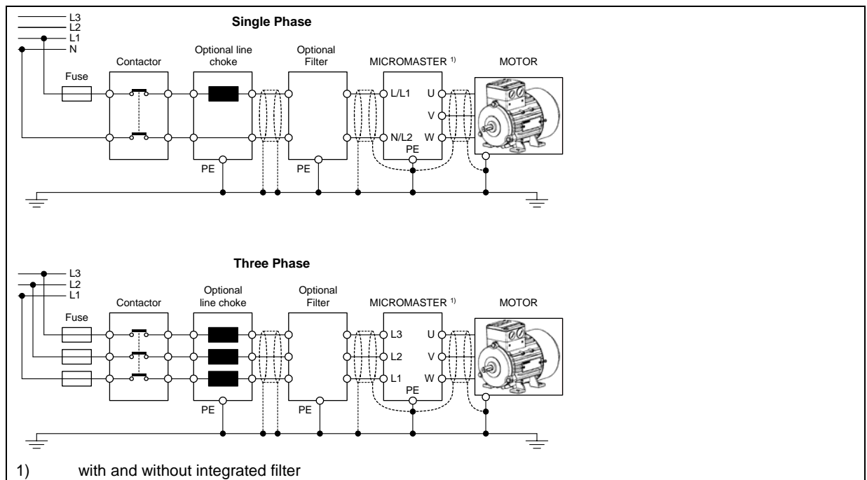
Fig. 4-5 Schematic diagram of the motor and line supply connections
