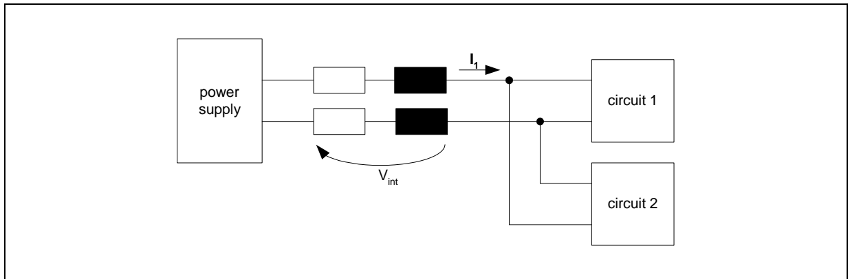
Fig. 3-3 Electrical coupling
