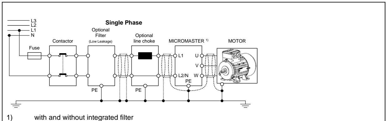
Fig. 4-4 Schematic diagram of the motor and line supply connections
