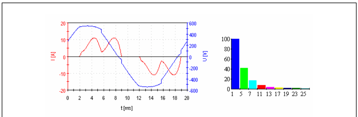
Fig. 3-2 Line supply voltage and current of a B6 rectifier
