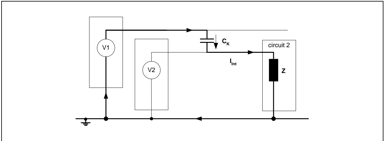
Fig. 3-4 Capacitive coupling for cables running in parallel
