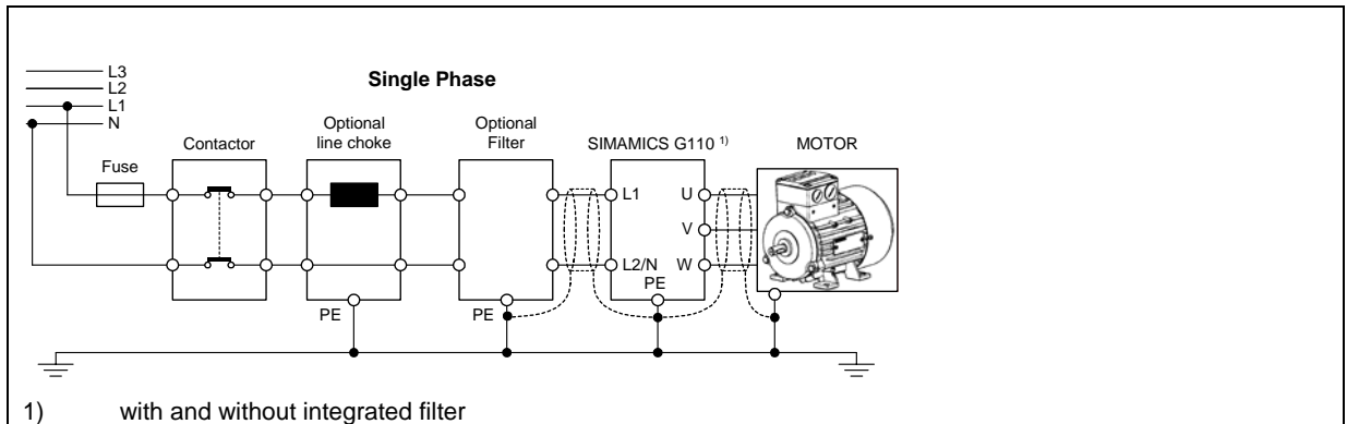
Fig. 4-3 Schematic diagram of the motor and line supply connections
