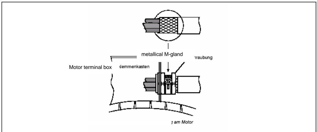
Fig. 4-10 Connecting the cable shield at the motor
