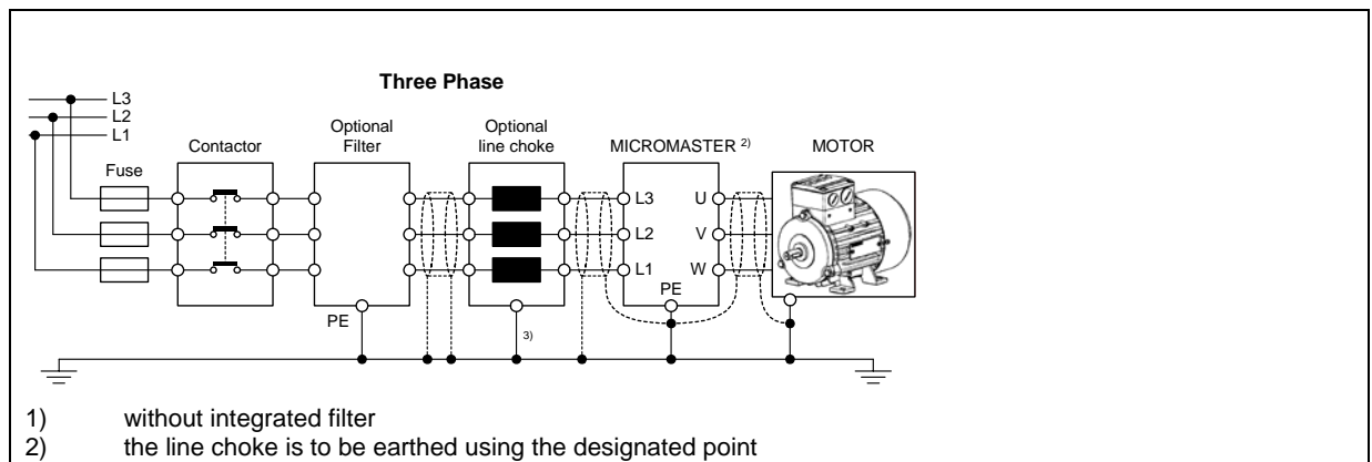
Fig. 4-6 Schematic diagram of the motor and line supply connections
