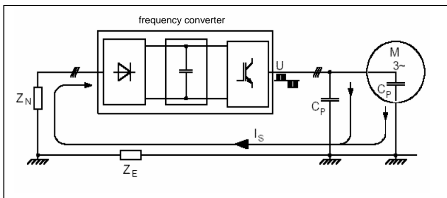
Fig. 3-1 Interference current I_s for unshielded motor feeder cables
