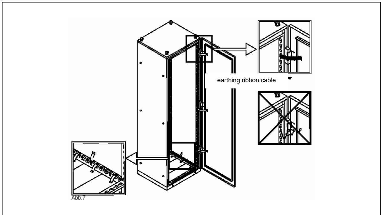
Fig. 4-2 Connecting housing parts
