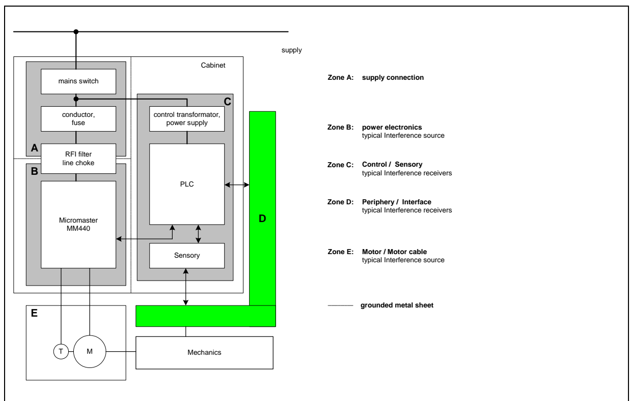
Fig. 4-1 Example for classifying a drive system according to various zones
