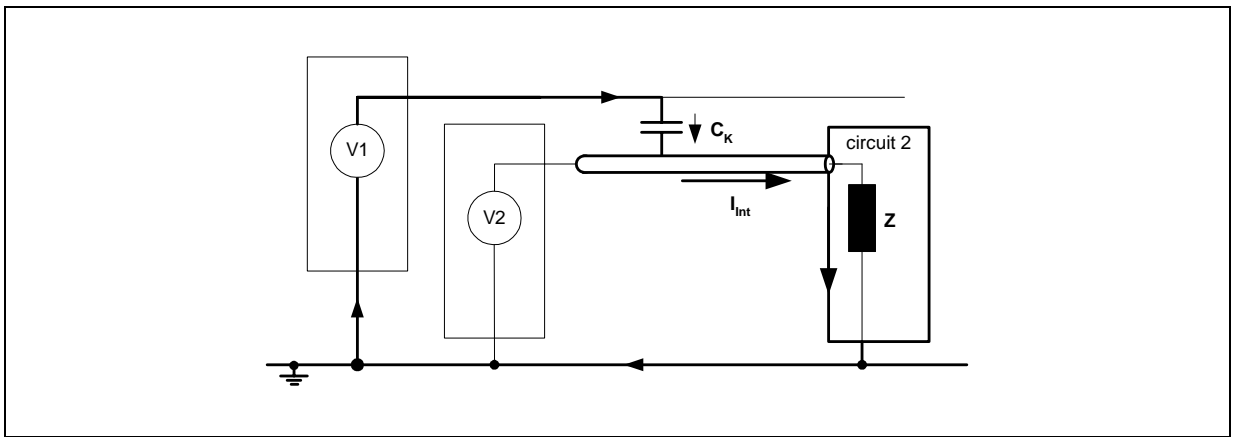
Fig. 3-5 Discharge interference current I_s
