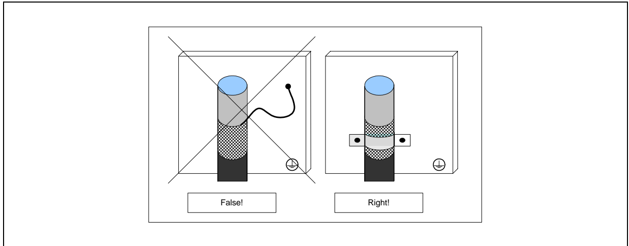
Fig. 4-9 Connecting the shield
