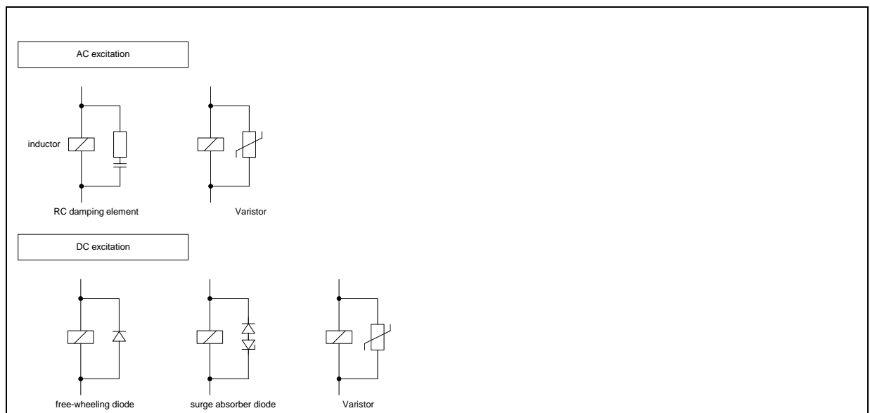
Fig. 4-7 Noise suppression elements
