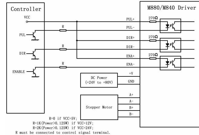
Figure 10: Typical connection
