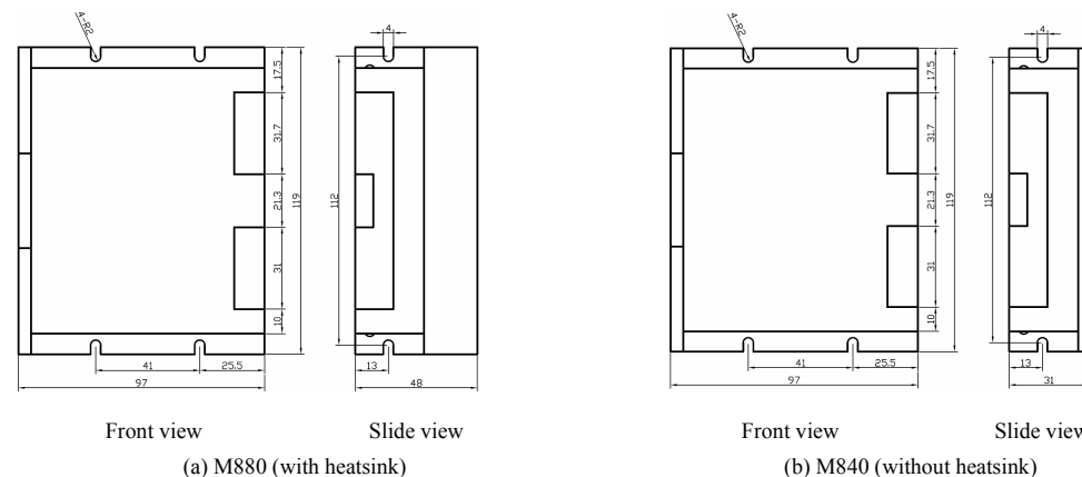
Figure 1: Mechanical specifications
