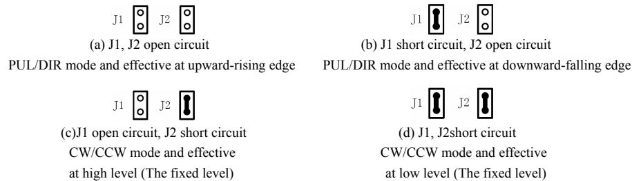
Figure 2: J1 and J2 jumpers
