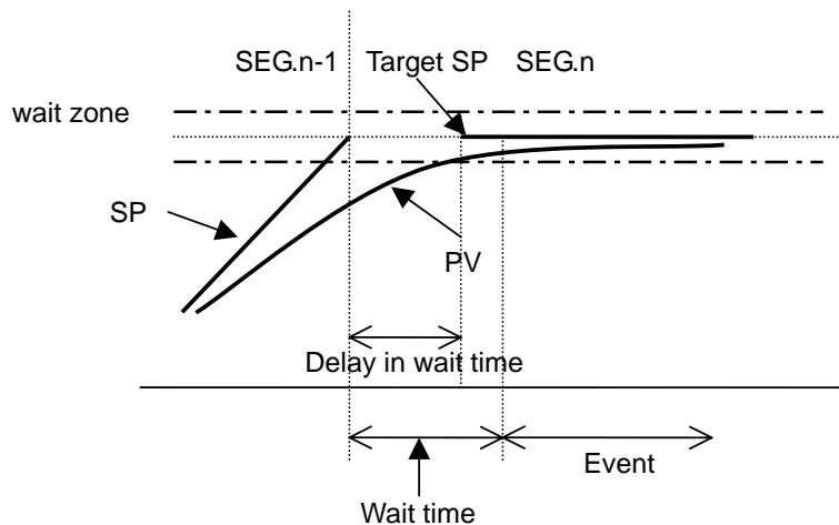
<Figure 7.6.1.2> Front Wait Operation (1)
