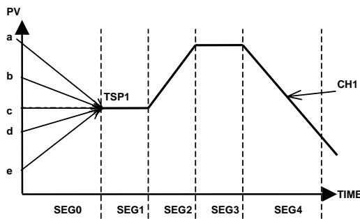
<Figure 7.1.6 (a)> Starting from the Temporary PV
