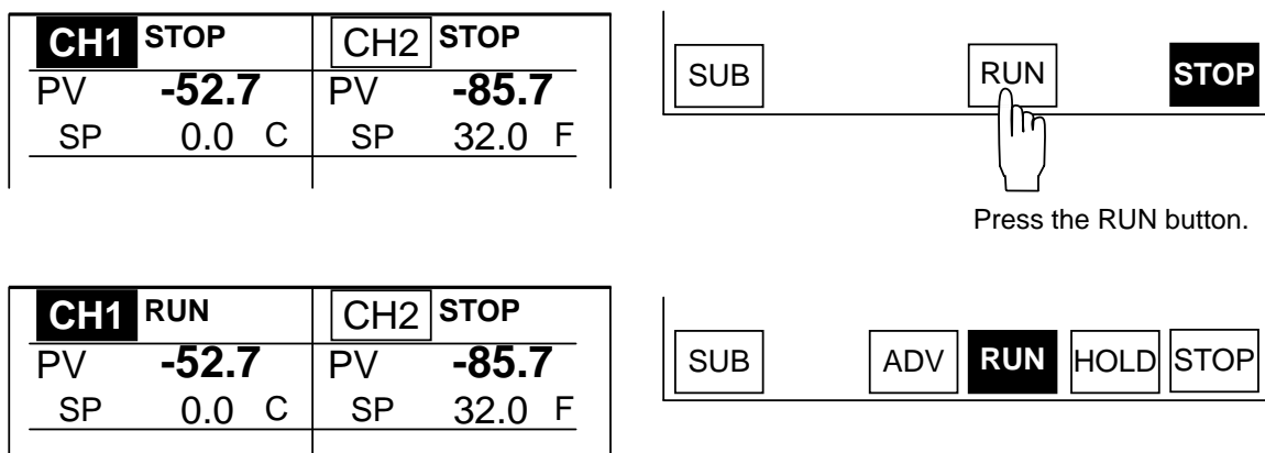
<Figure 5.1.2> Displaying the RUN Operation Status
