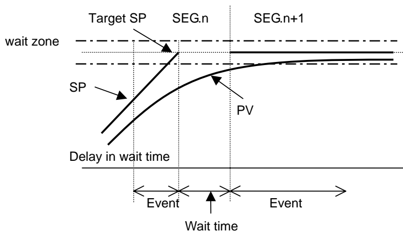
<Figure 7.6.1.5> Rear Wait Operation (2)
