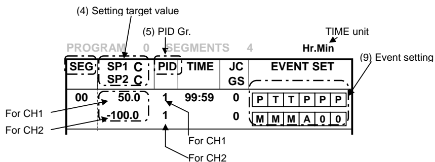
<Figure 7.2.2.2> Displaying the Segment Data
