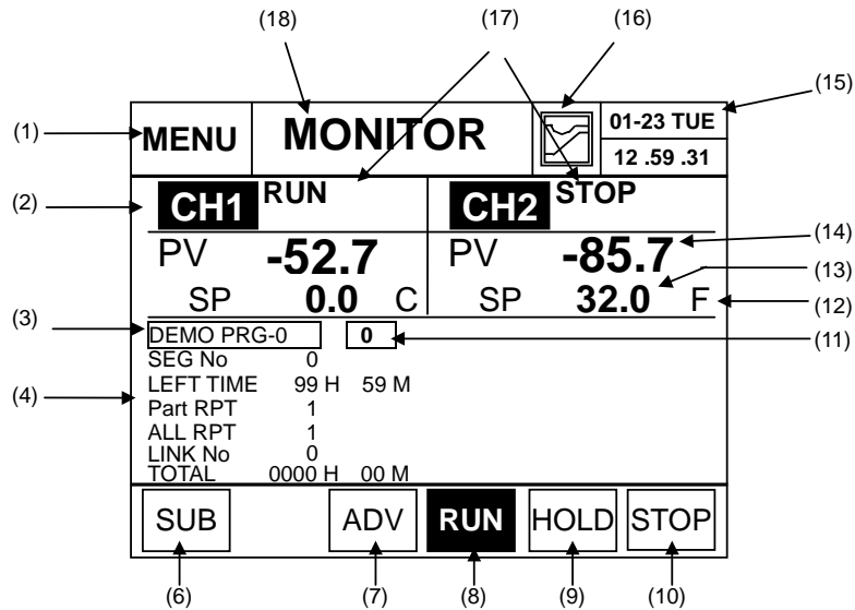
<Figure 5.1.13> MONITOR Screen (Program Operation, Synchronous Mode)
