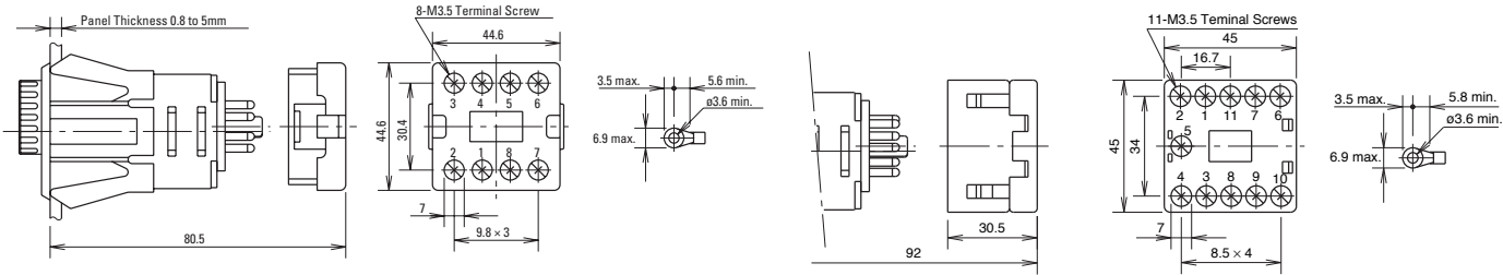
GT3 Timer, 8-Pin with SR6P-M08G
