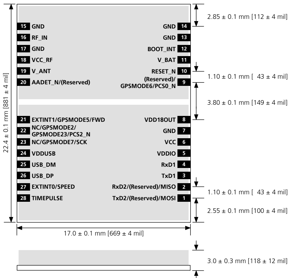
Figure 2: Dimensions
