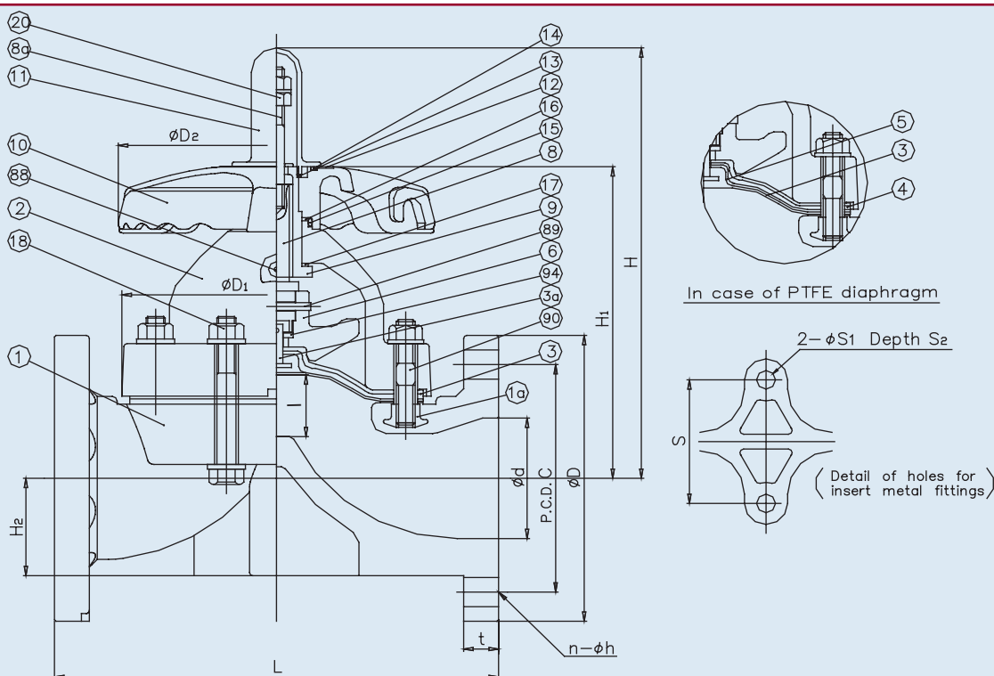
Dimensions Type-14 Flanged (Sizes 2-1/2" - 4") (in.)
