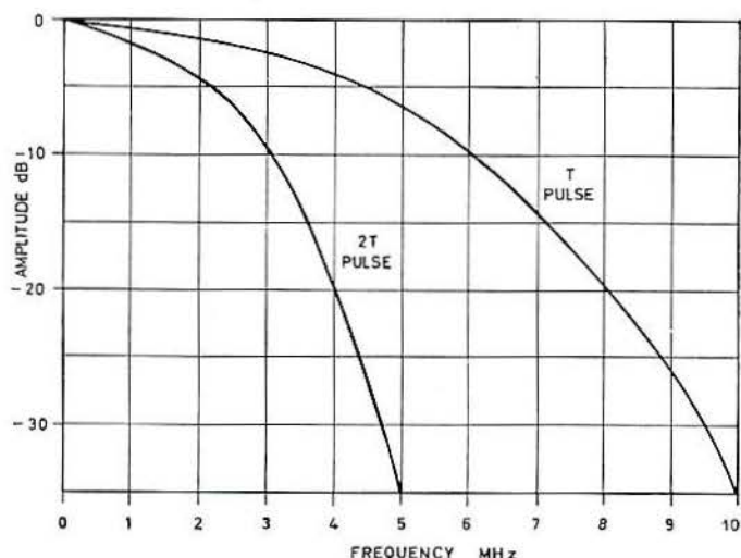
Fig. 2. Spectrum of a sine-squared pulse.
