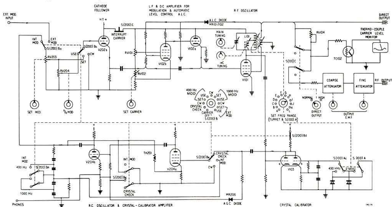
Functional Diagram of TF 144H/4
