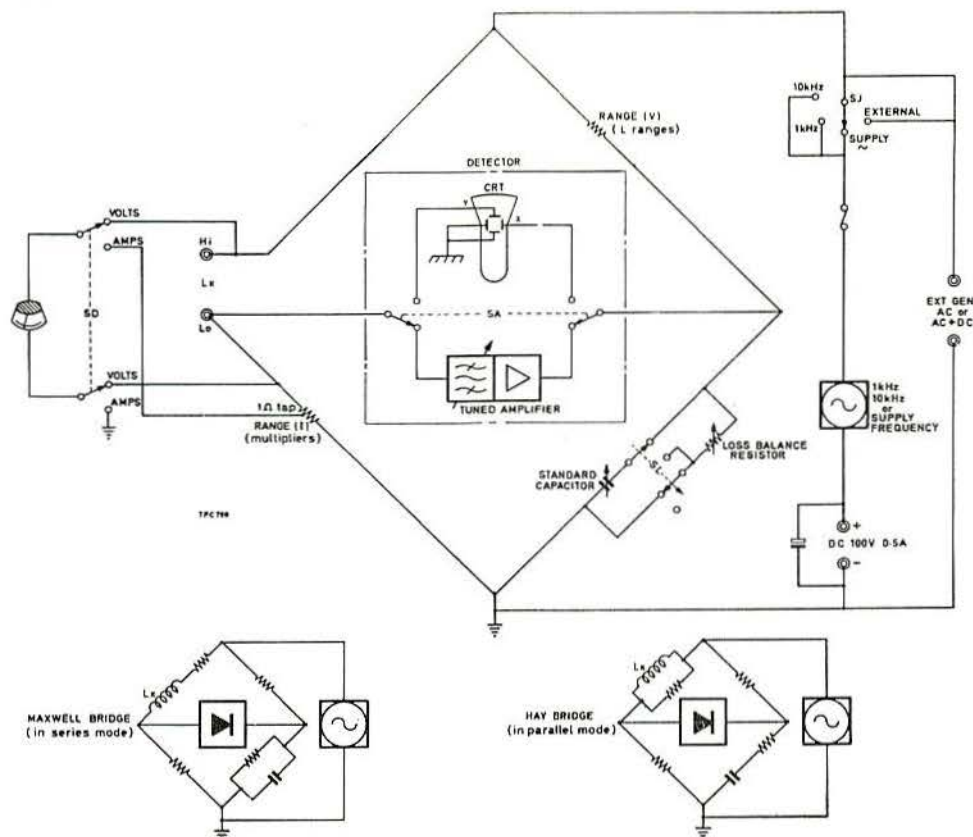
Functional diagram
