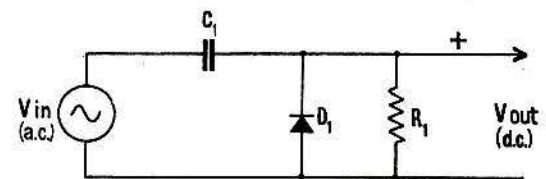
Fig. 4 Peak Detector (parallel configuration).
