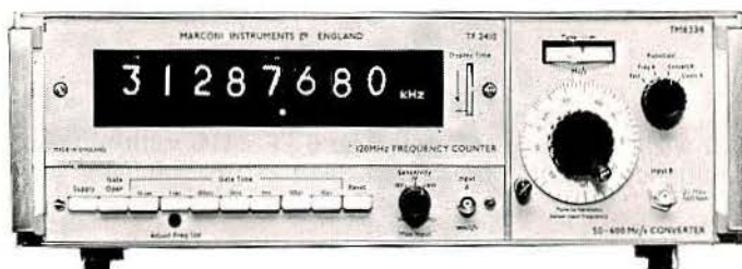
TF 2410 with plug-in Converter TM 8334
