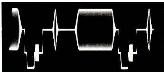
Chrominance Waveform on Pedestal, 525 line TF 2905/9
