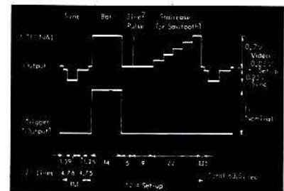
Waveform for general assessment (monochrome) with internal trigger
