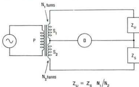
Fig. 2 Transformer-ratio-arm bridge.
