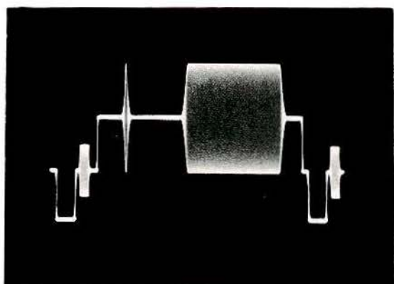
Fig. 5. Chrominance sine squared pulse and bar.
