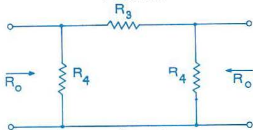
pi Network
