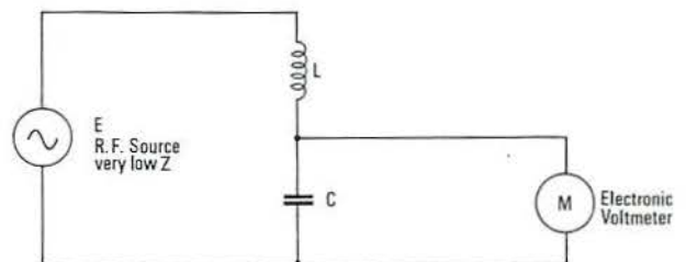
Fig. 4 Functional arrangement of circuit magnification meter.
