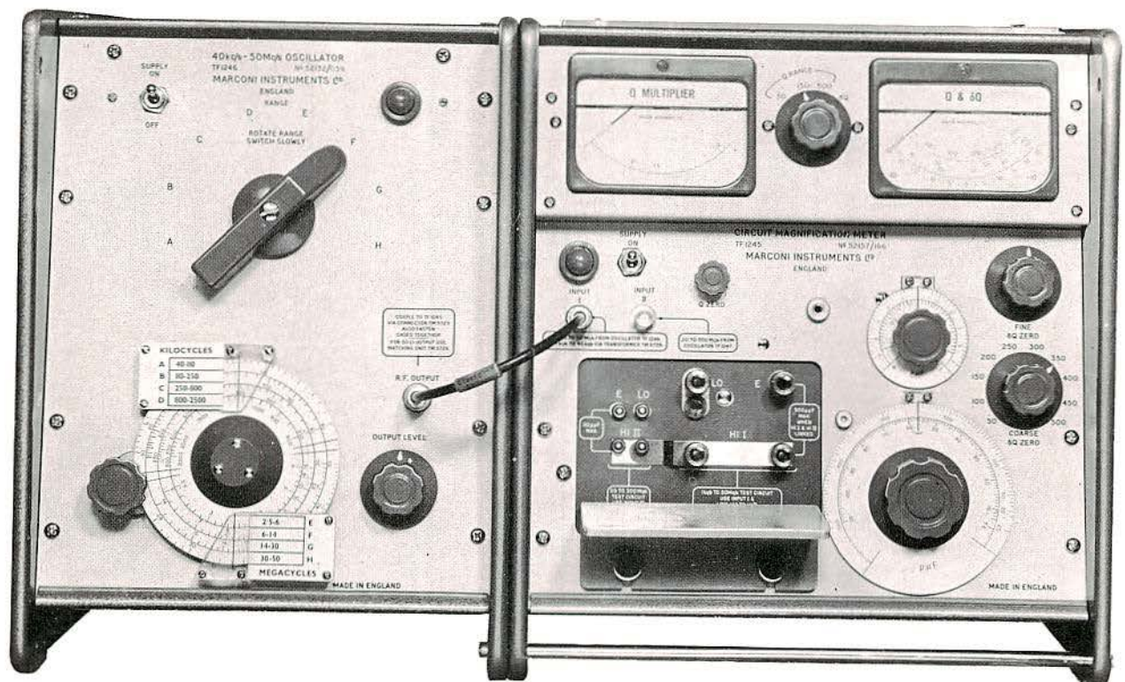
Q Meter and TF 1246 Oscillator
