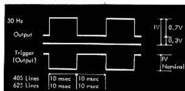
Waveform for l.f. response measurement
