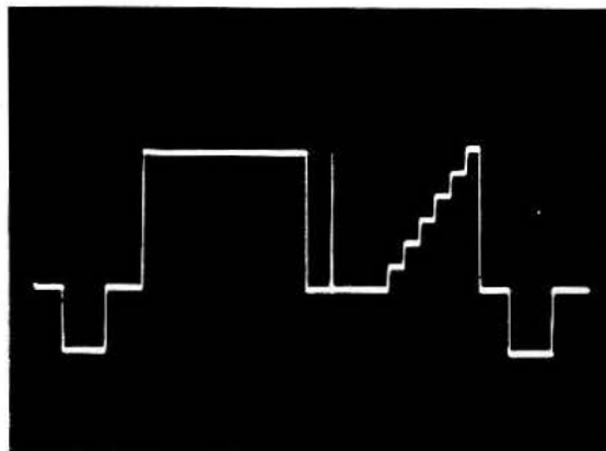
Fig. 10. Monochrome insertion signal for 625 lines.
