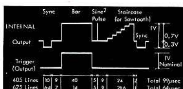
Waveform for general assessment (monochrome) with internal trigger
