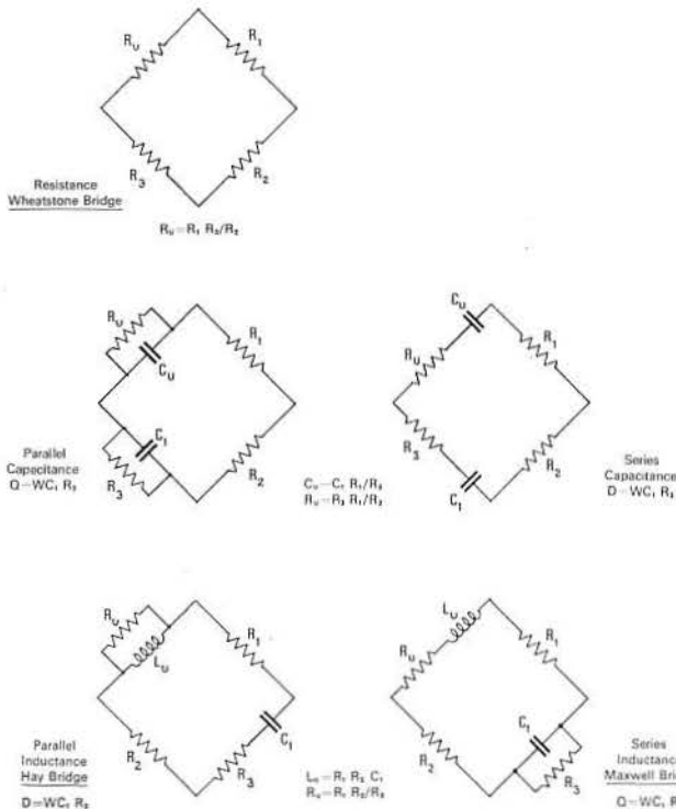
Fig. 1 Impedance-ratio-arm bridges.
