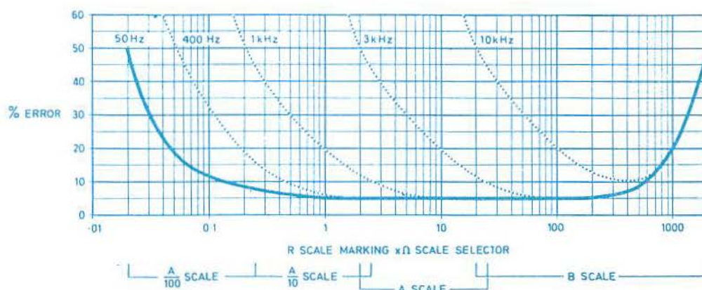
Typical resistance scale accuracy at representative frequencies.
