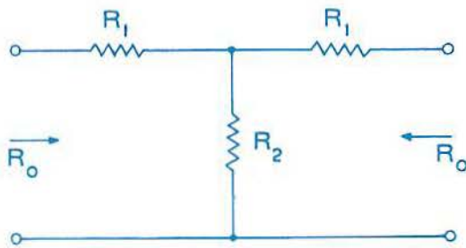
T Network
