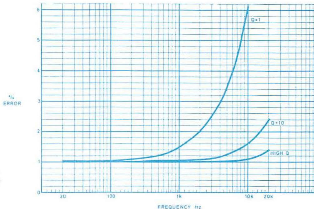
Inductance Accuracy This graph shows the percentage of error of the inductance measurement at representative values of Q.
