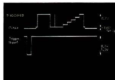
Monochrome insertion waveform from external trigger
