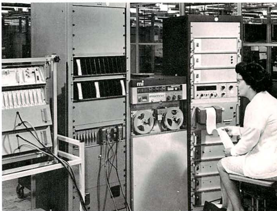
One of several "Autotest" L.F. measurement systems installed to check P.C.M. terminal equipment.
