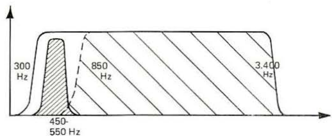
B.P.O. FILTER CHARACTERISTICS.
