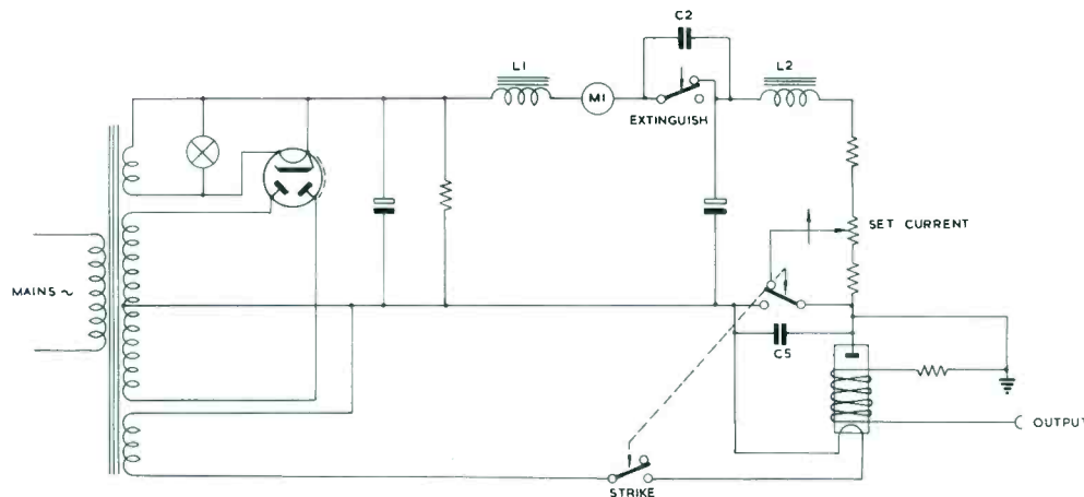
Fig. 2 Functional diagram of Noise Generator, Type TF 1301
