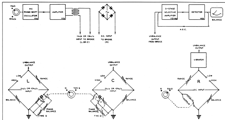
Functional Diagram of TF 868B
