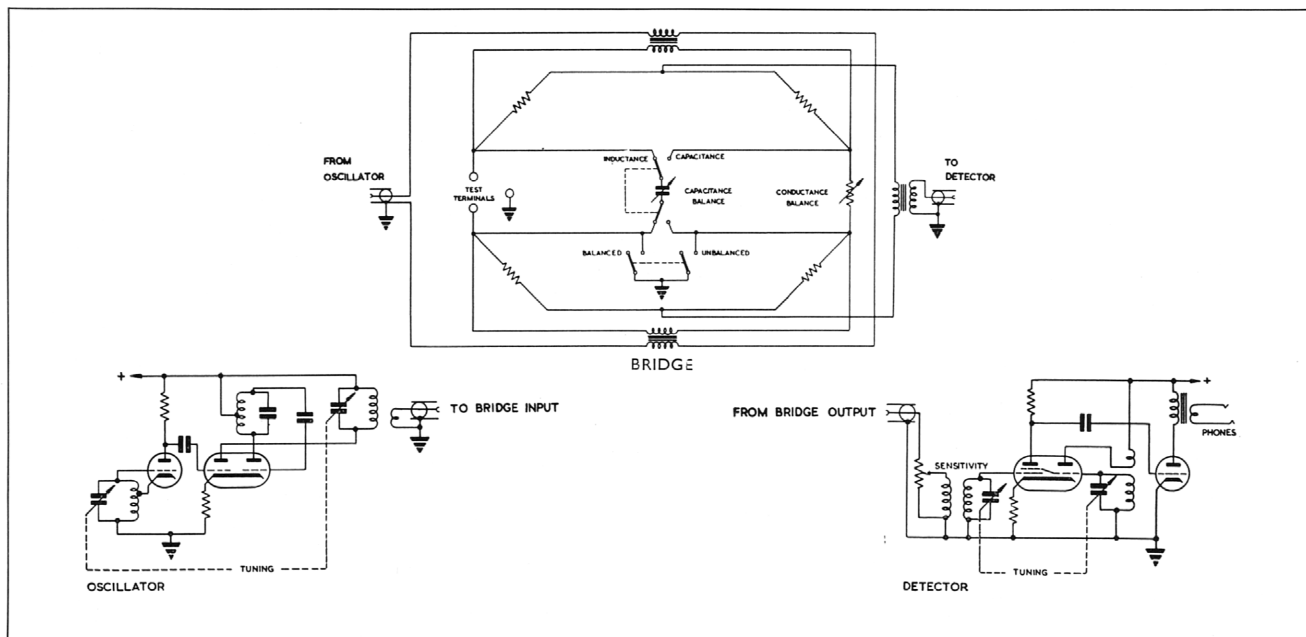
Functional Diagram of OA 199A/2
