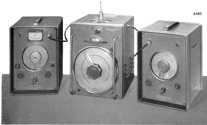
V.H.F. Bridge Detector Type TF 1275
