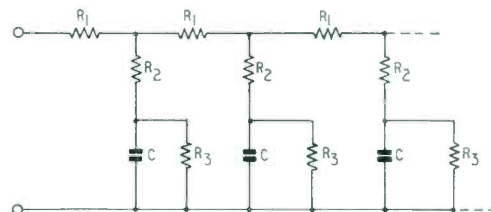
Fig. 2. General representation of an electrolytic capacitor
