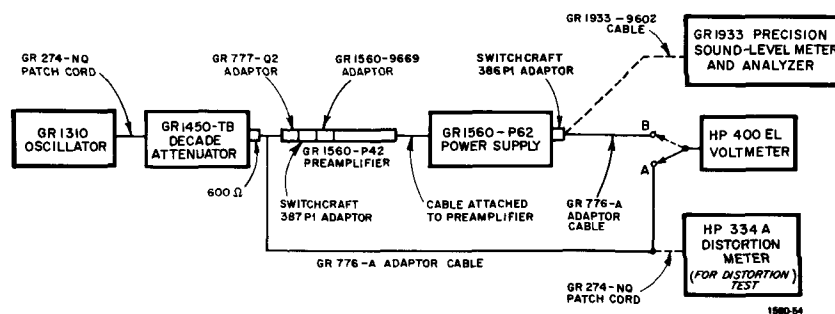
Figure 4-13. Test setup for minimum-performance checks.
