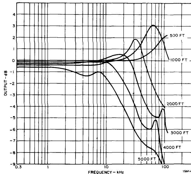
Figure 4-8. Measured cable loss of the Preamplifier vs cable length for Belden #8771 cable. Preamplifier gain is \times 1 , powered from the receiver end.
