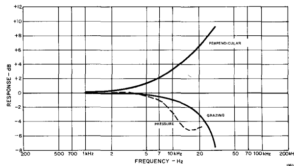
Figure 3-13. Corrections to be added algebraically to the random-incidence response to obtain the perpendicular- or grazing-incidence free-field response, or pressure response for the ½-in. electret microphone, Type 1962-9601.
