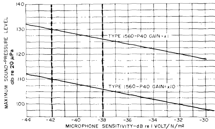
Figure 7-4. Maximum sound-pressure level that can be measured with a Type 1560-P40 Preamp-fier-and-microphone combination. The sensitivities of Types 1971-9605 and -9606 Microphones will fall between the dotted lines. Allowance is made for a peak-to-rms ratio of 14 dB. For a sine-wave acoustic signal, the maximum level can be increased by 11 dB.
