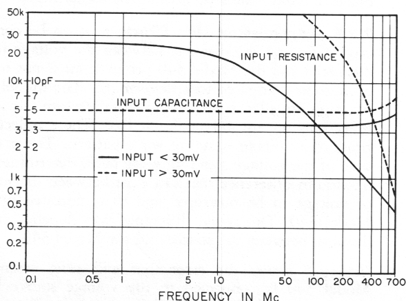
Fig. 4. Model 340 Input Impedance
