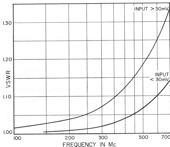
Fig. 6. Model 5340 VSWR
