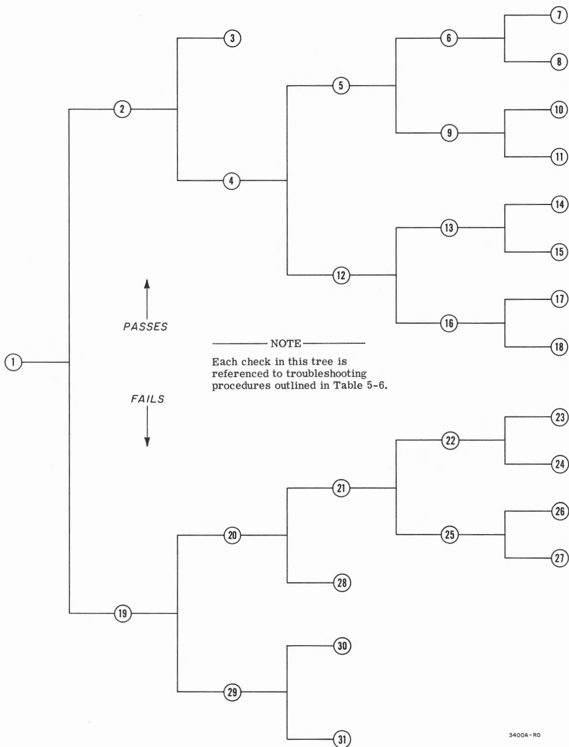
Figure 5-5. Troubleshooting Tree
