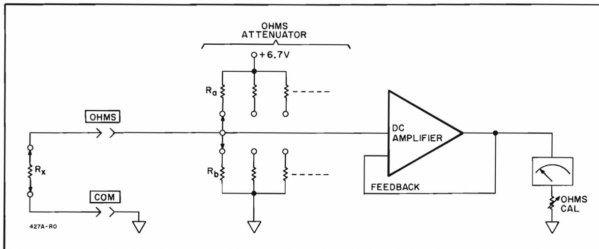
Figure 4-3. Ohms Operation
