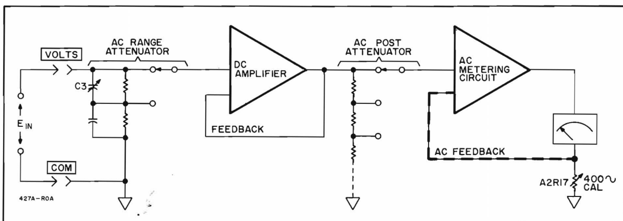
Figure 4-4. AC Operation
