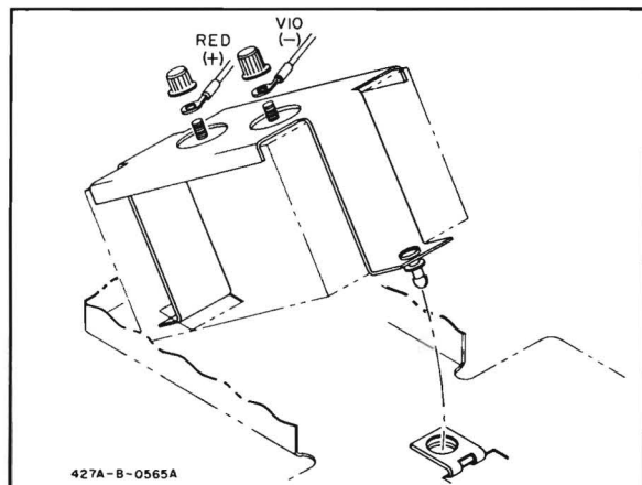
Figure 5-7. Battery Replacement
