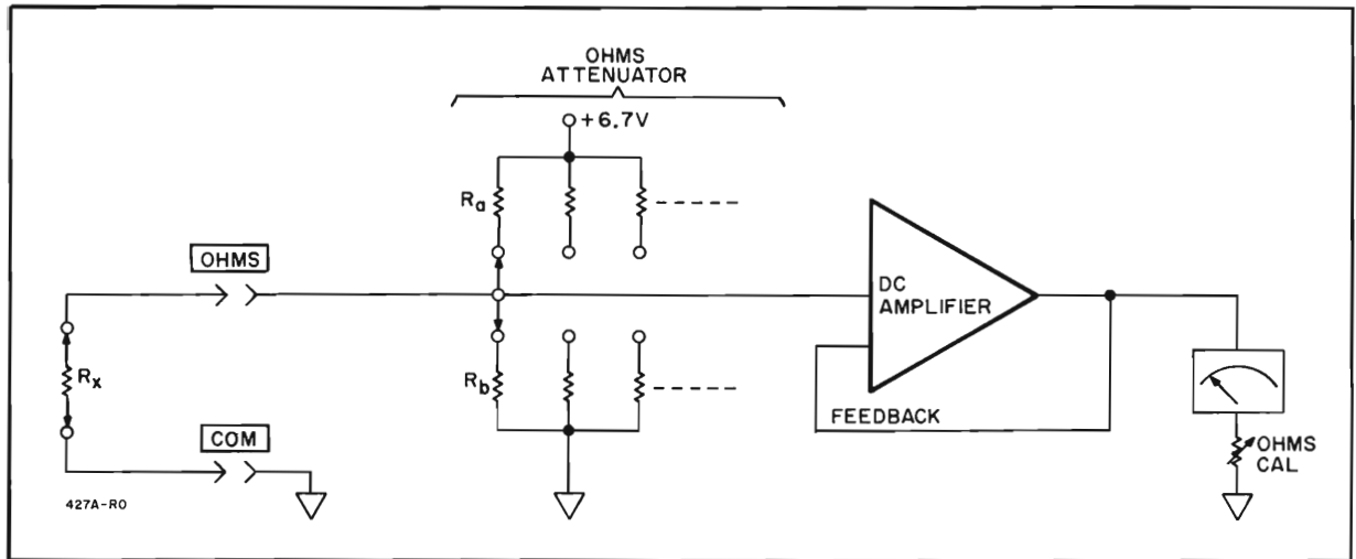
Figure 4-3. Ohms Operation
