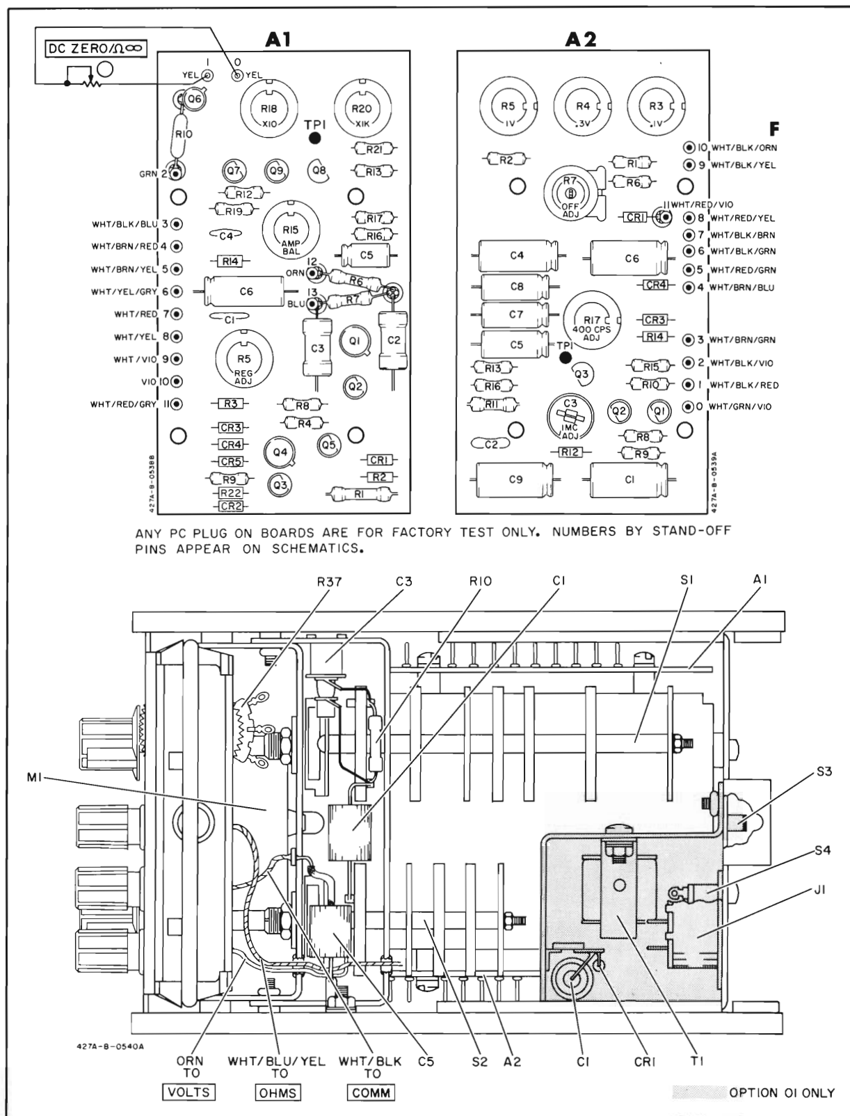
Figure 6-2. Component Location
