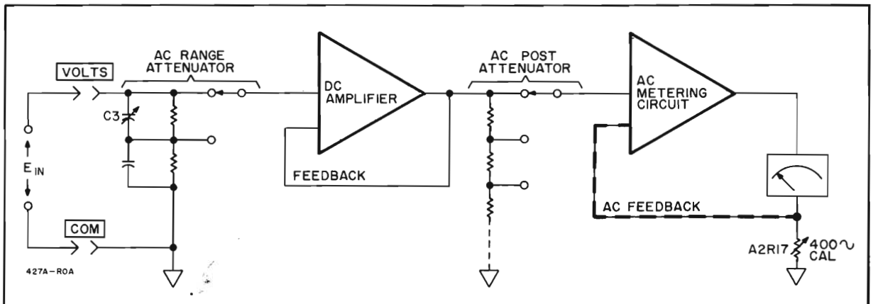
Figure 4-4. AC Operation
