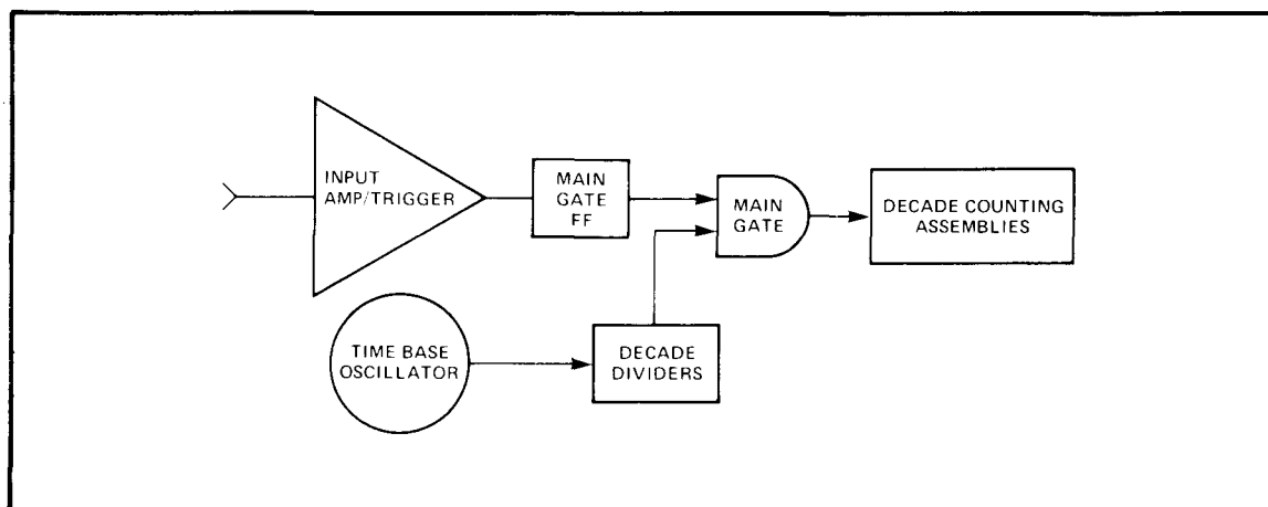
Figure 3-2. Measuring Period
