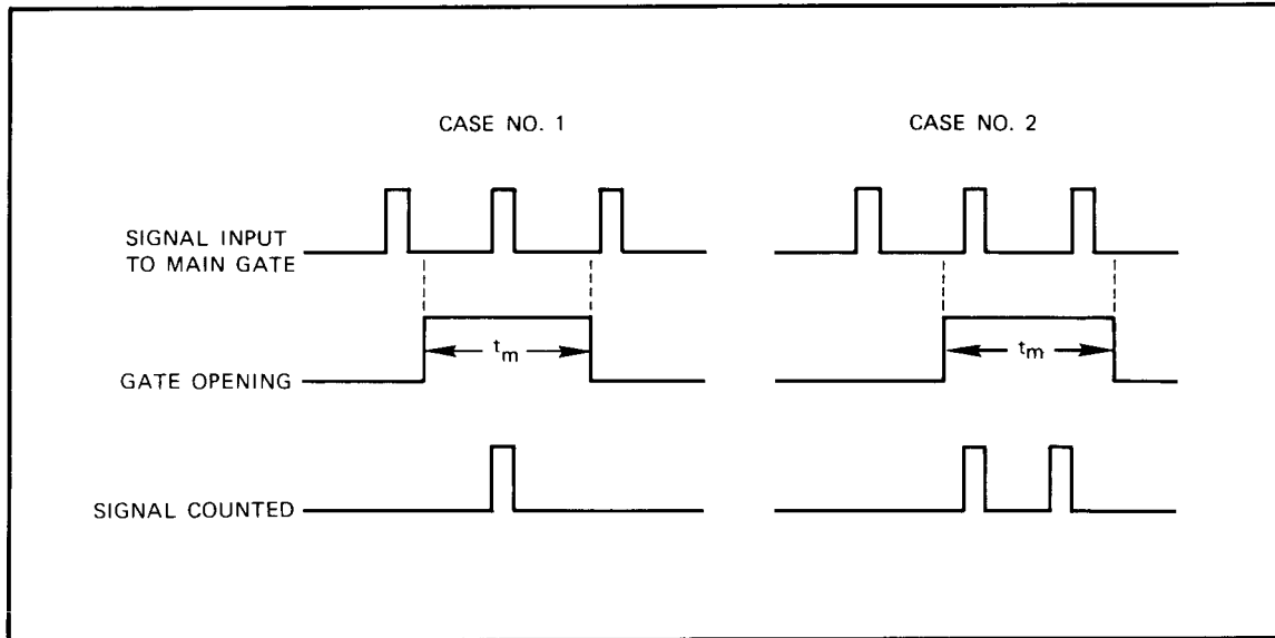
Figure 3-6. +1 Count Ambiguity
