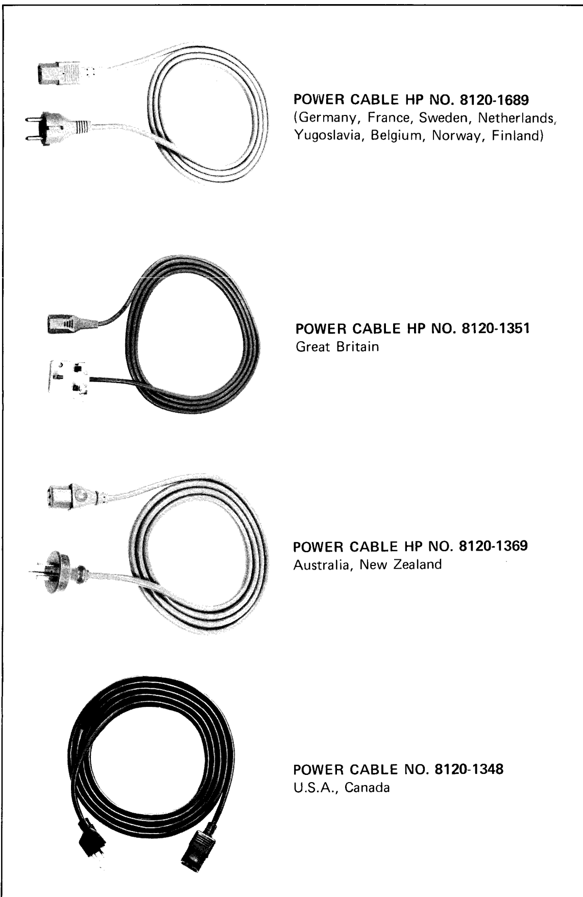
Figure 2-1. Power Cables
