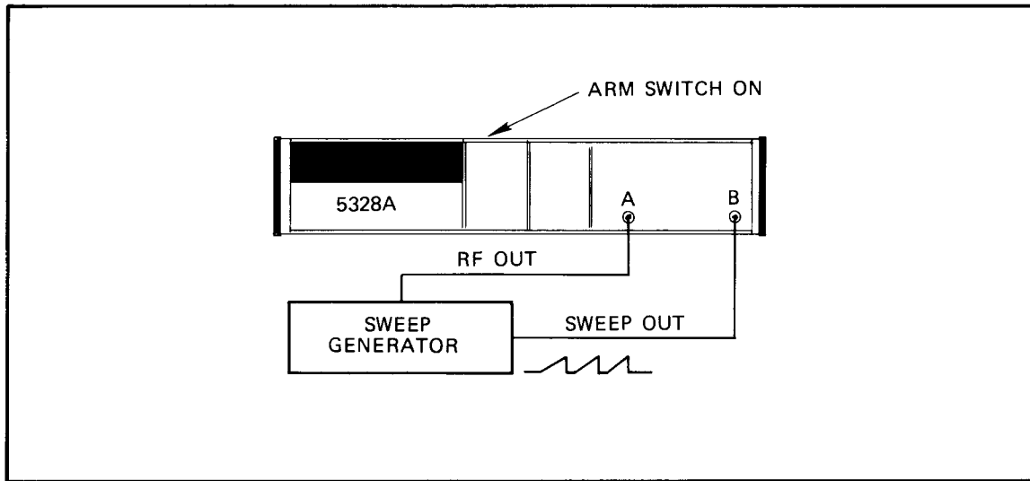
Figure 4-1. Measuring Linearity
