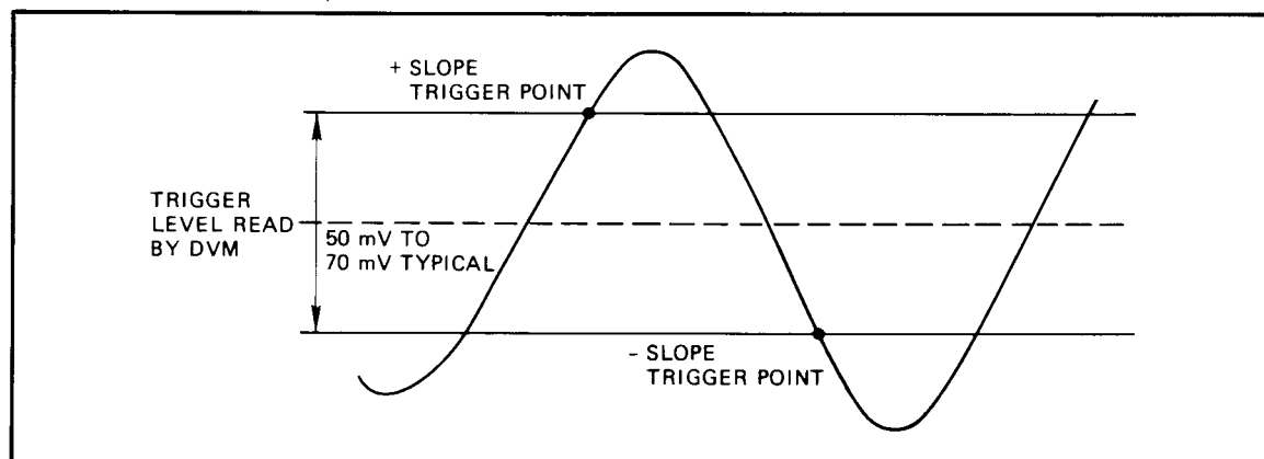
Figure 3-18. Hysteresis Band
