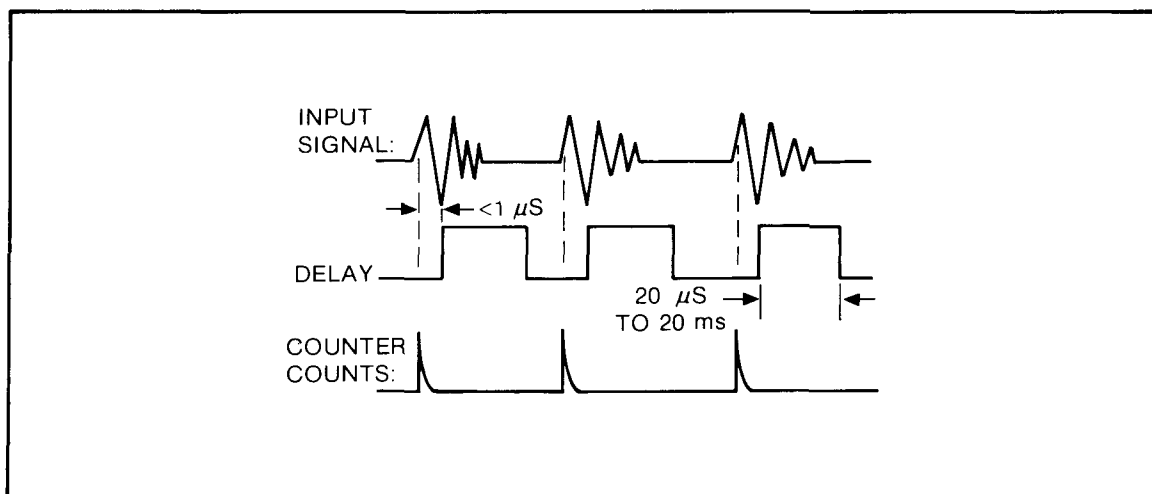
Figure 3-19. Delay Mode
