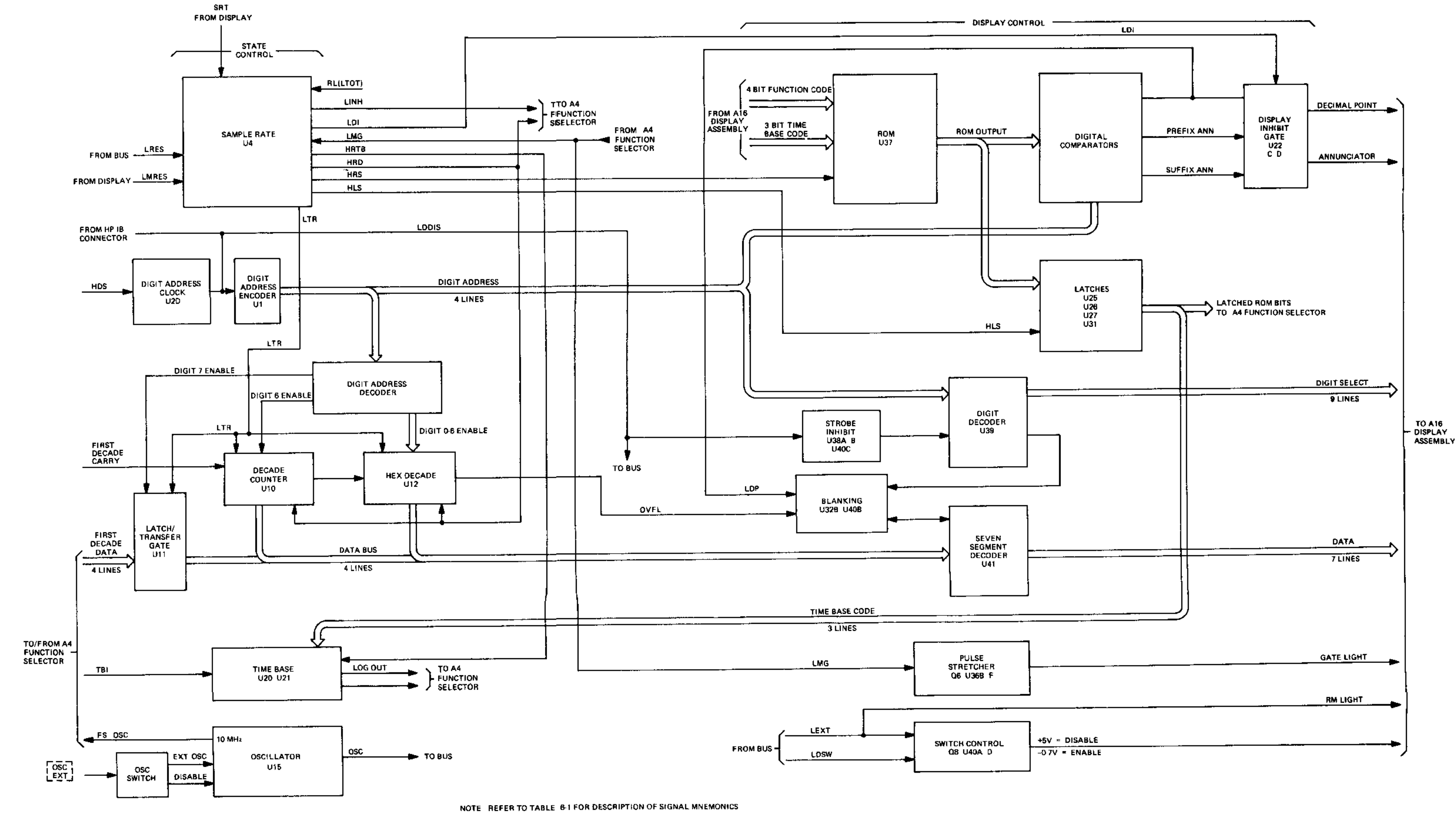
Figure 8-6. A1 Motherboard
