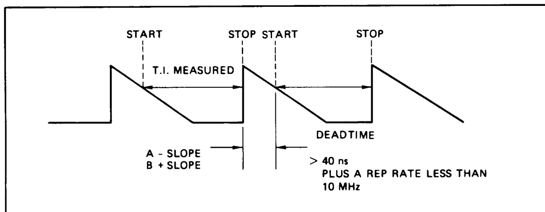
Figure 3-3. Deadtime
