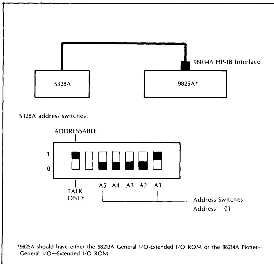
Figure 5-6. System Configuration
