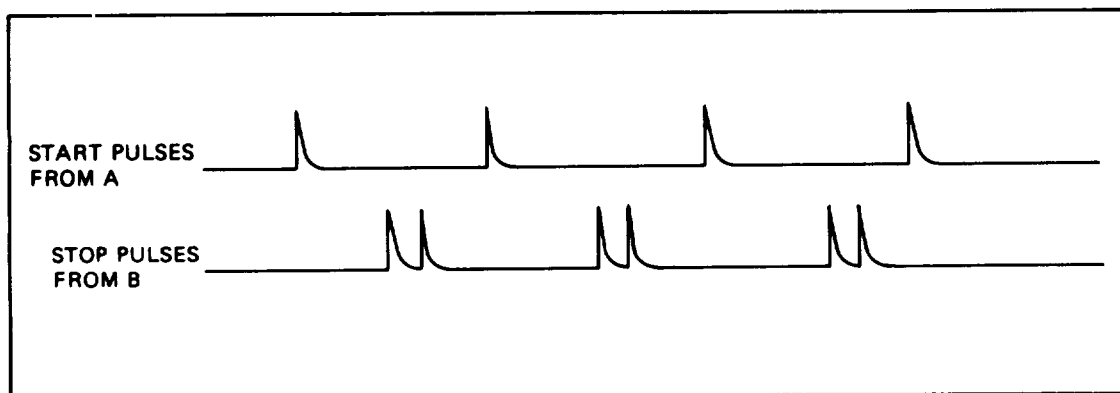
Figure 3-4. Multiple STOP Pukes
