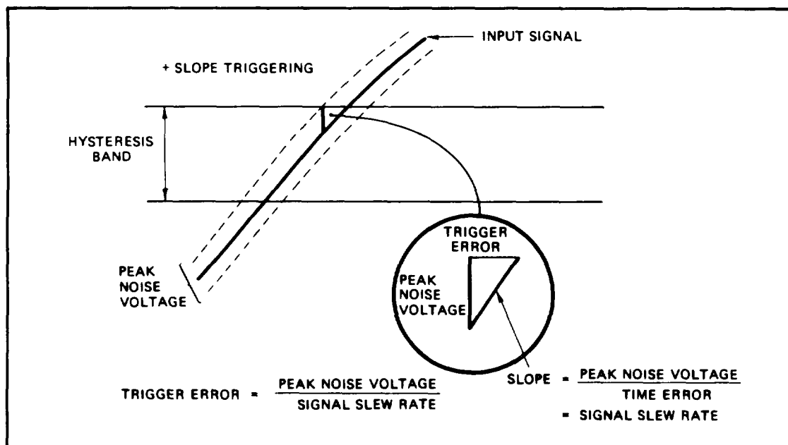
Figure 4-7. Trigger Error
