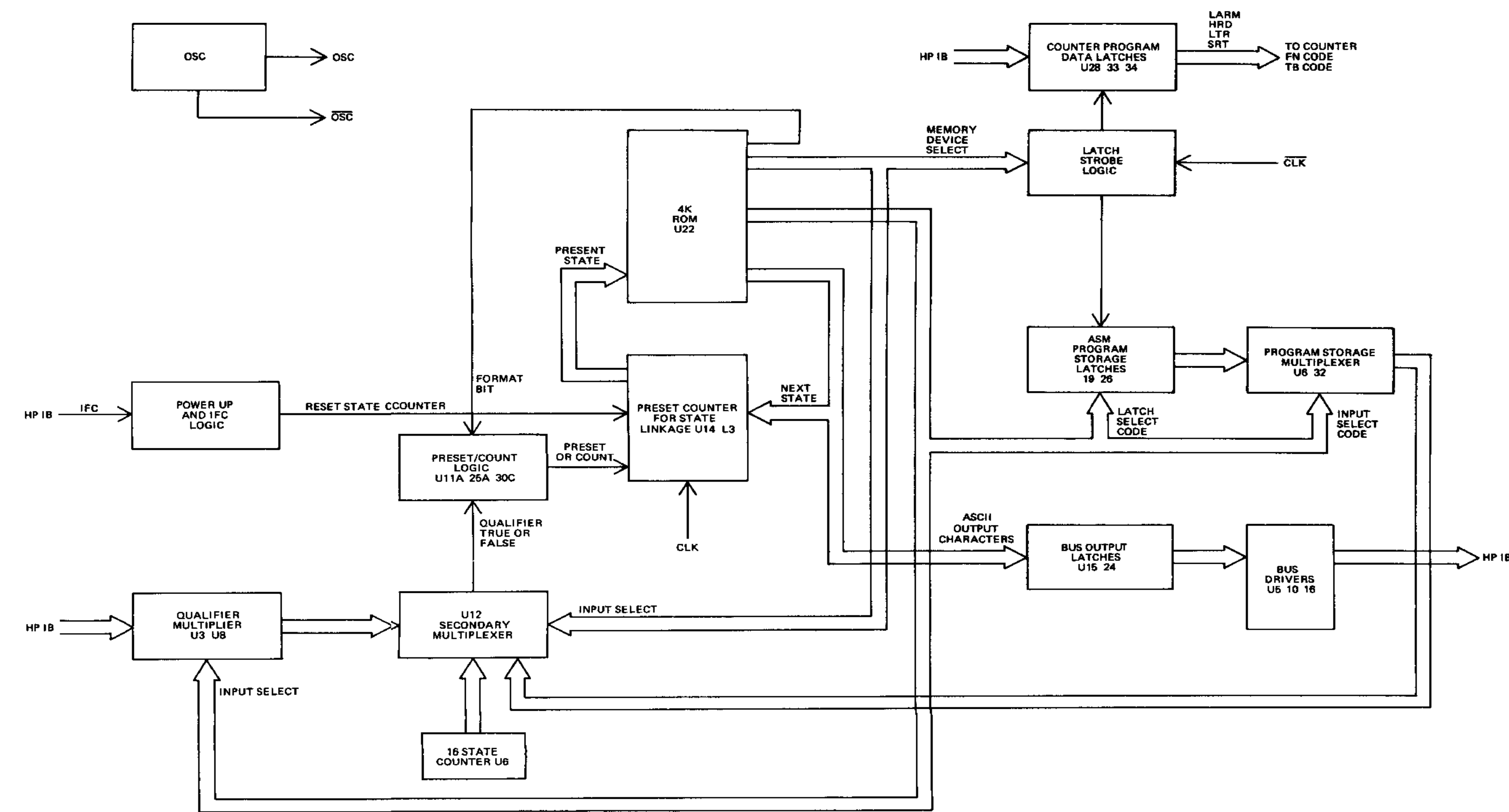
Figure 8-21. A15 HP-IB Interface Block Diagram
