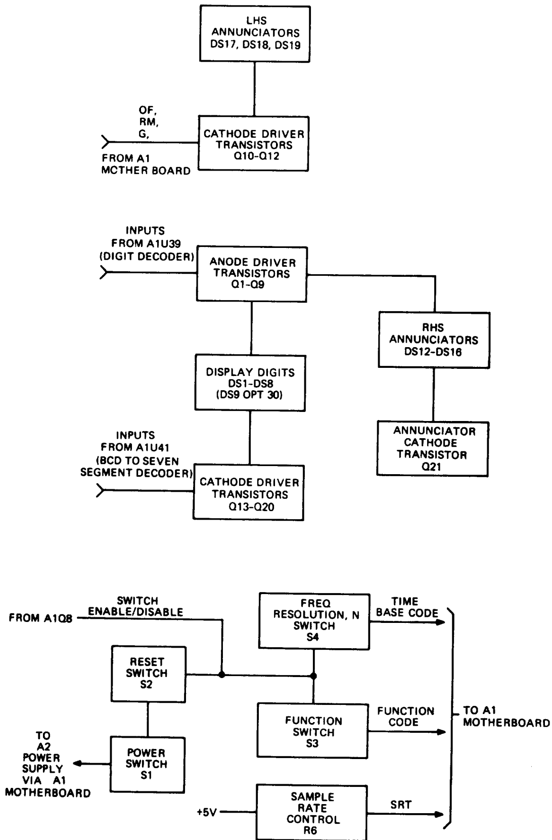
Figure 8-23. A16 Display Block Diagram
