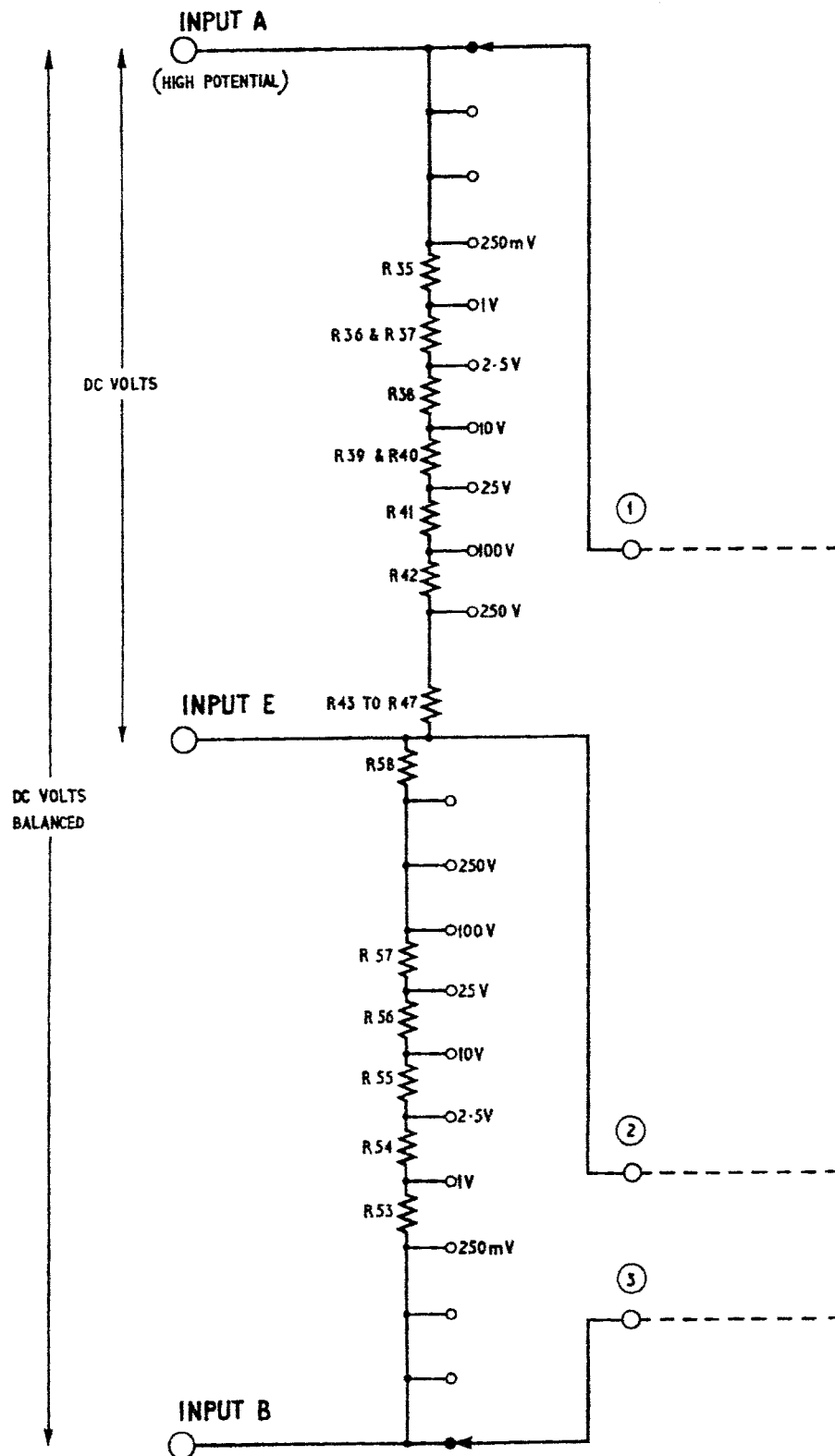
Fig.10.DC volts and DC volts (balanced) measuring circuit
