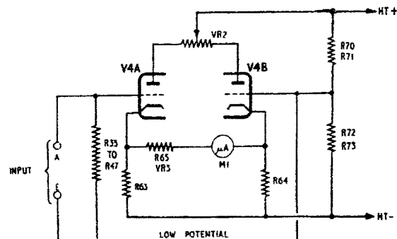
Fig. 1. Basic DC millivoltmeter circuit
