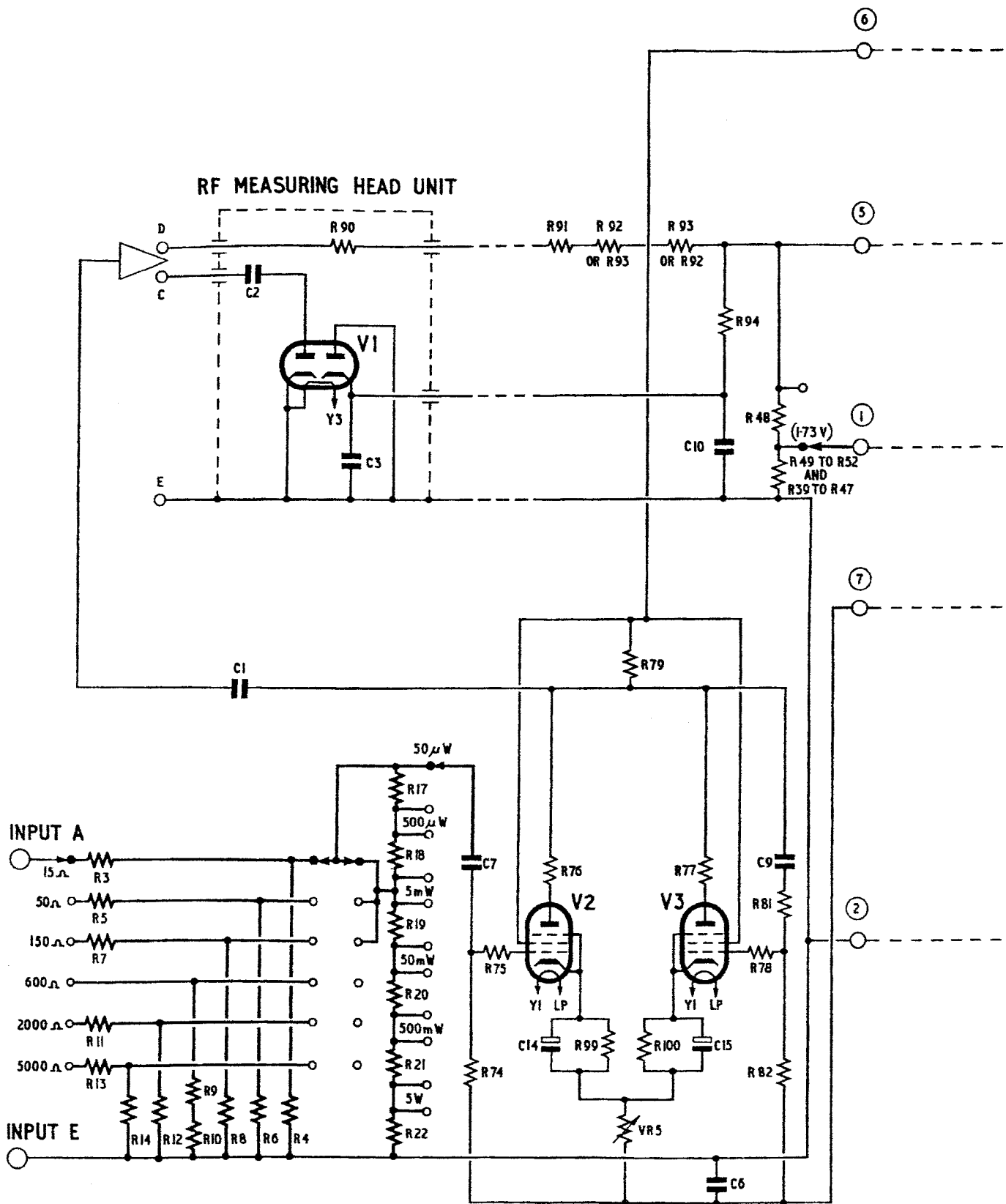
Fig. 17. Watts measuring circuit
