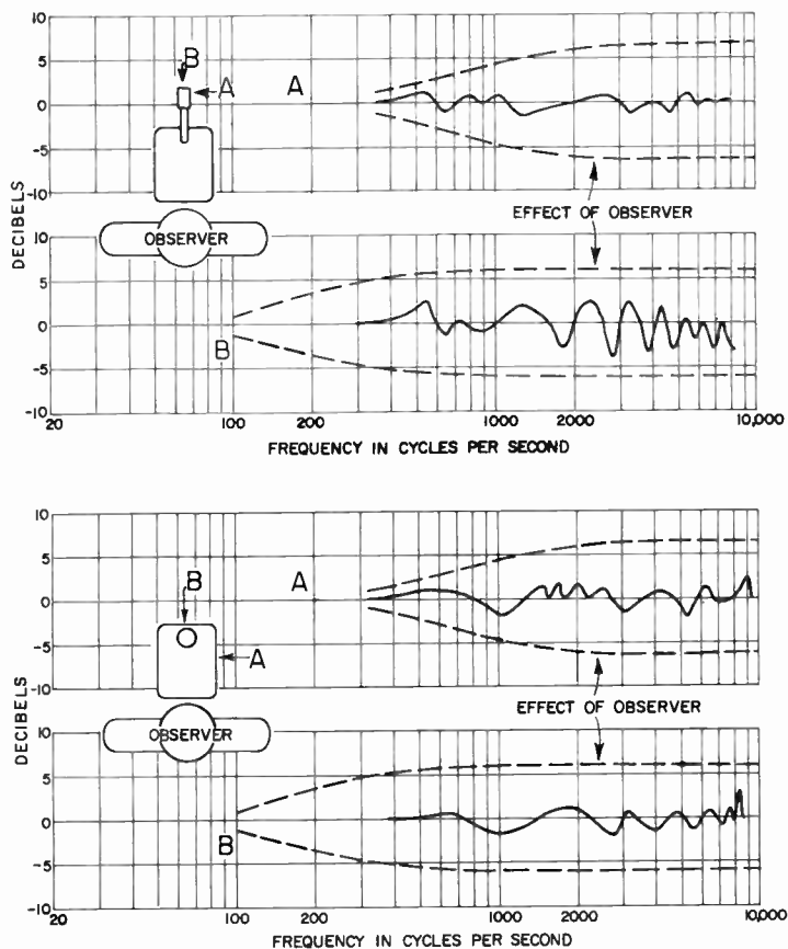
Figure 6-10. Effect on frequency response as a result of using the microphone directly on the swivel post of the instrument (in two positions) without an observer present and the extent of the effect with an observer present. The decibel readings were obtained using a single-frequency, plane, acoustic wave in an anechoic chamber, and they are the differences between the response under conditions shown and the response of the microphone alone.
