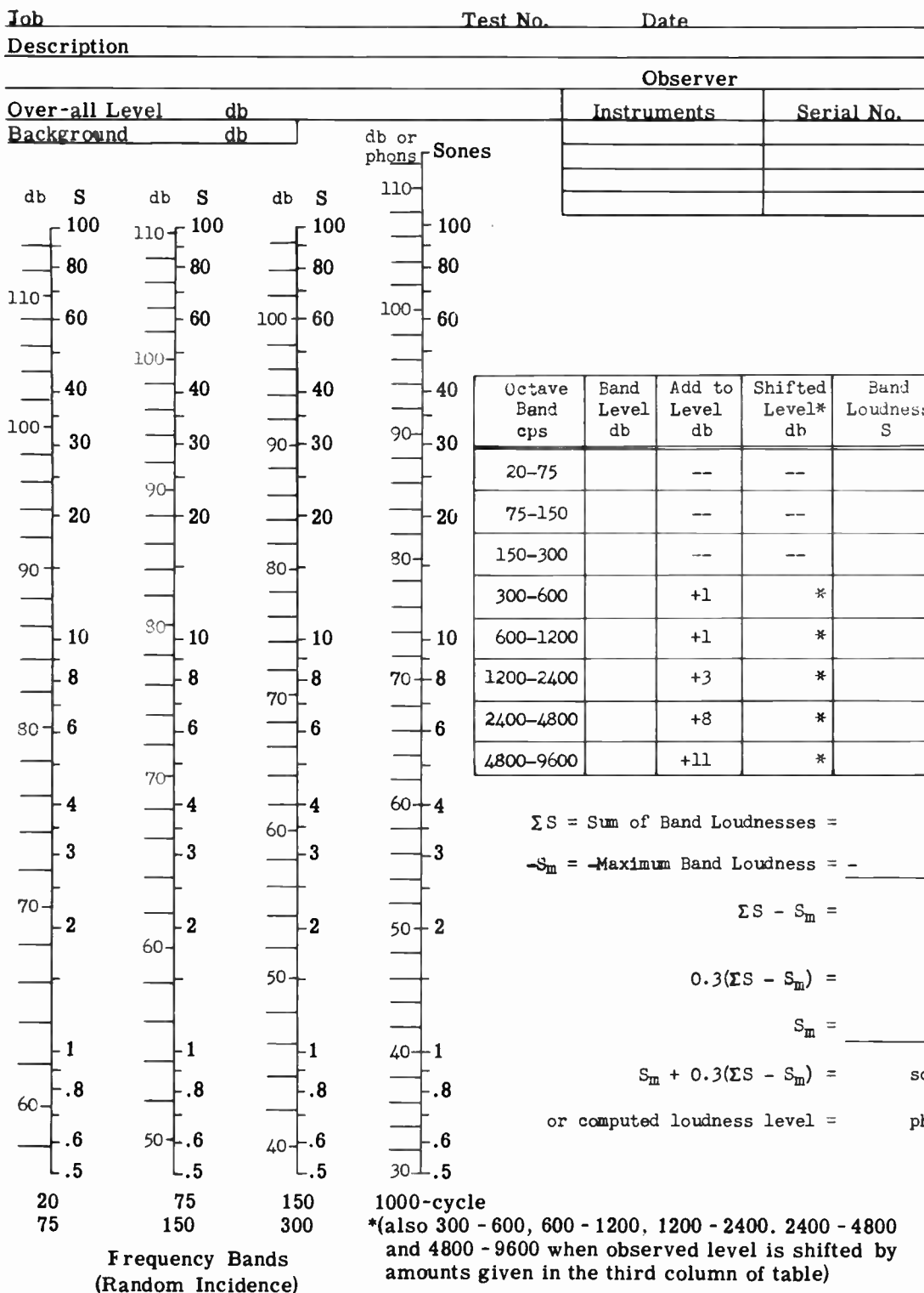
Figure 8-1. Chart for calculating loudness level from an octave-band analysis of a noise. The noise has been assumed to be coming at the listener from many directions (random incidence).
