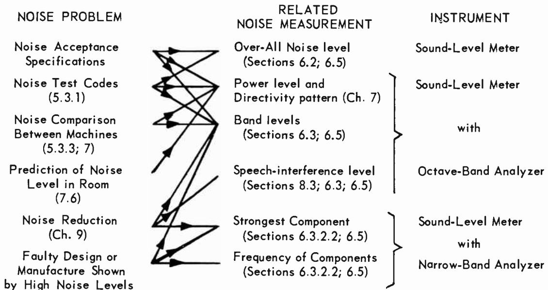
Figure 5-9. A summary of measurements on noisy devices. As above, the arrows suggest the noise measurements that may help in understanding the noise problem and in doing something about it.
