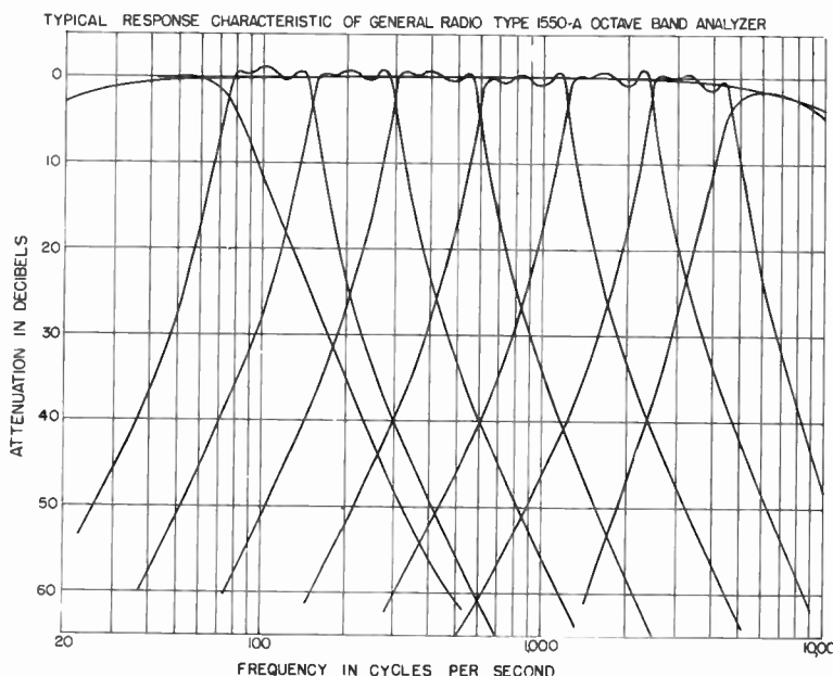
Figure 6-4. Typical response characteristics of the Type 1550-A Octave-Band Noise Analyzer.
