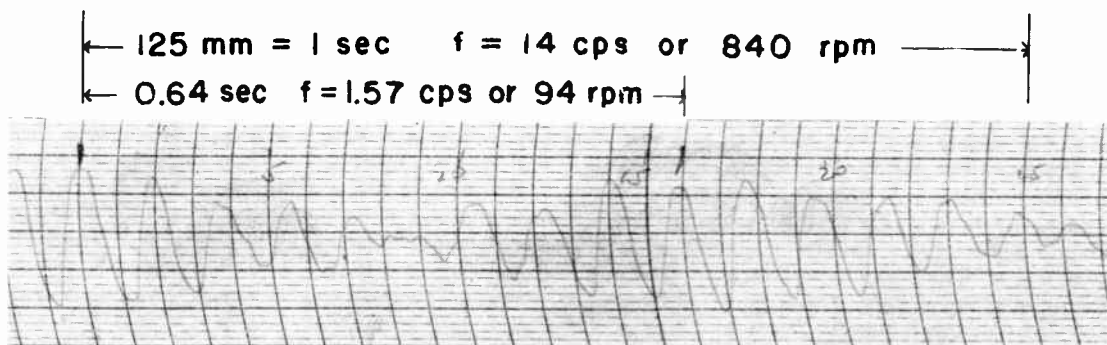
Figure 12-8. Record taken under the same conditions as Figure 12-7 except with a chart speed of 125 millimeters per second.
