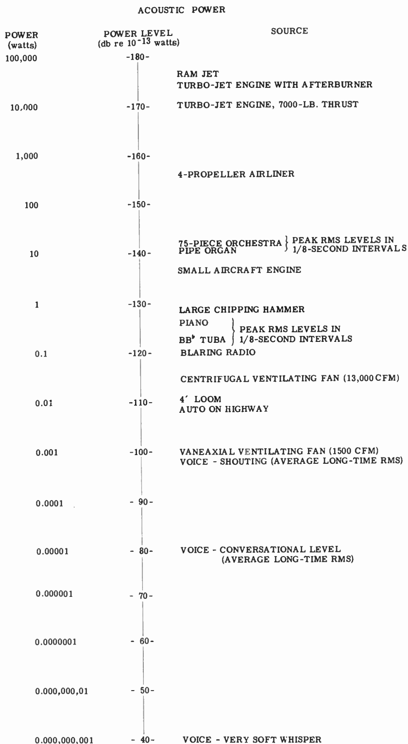
Figure 2-2. Typical power levels for various acoustic sources. These levels bear no simple relation to the sound levels of Figure 2-1. See Chapter 7.
