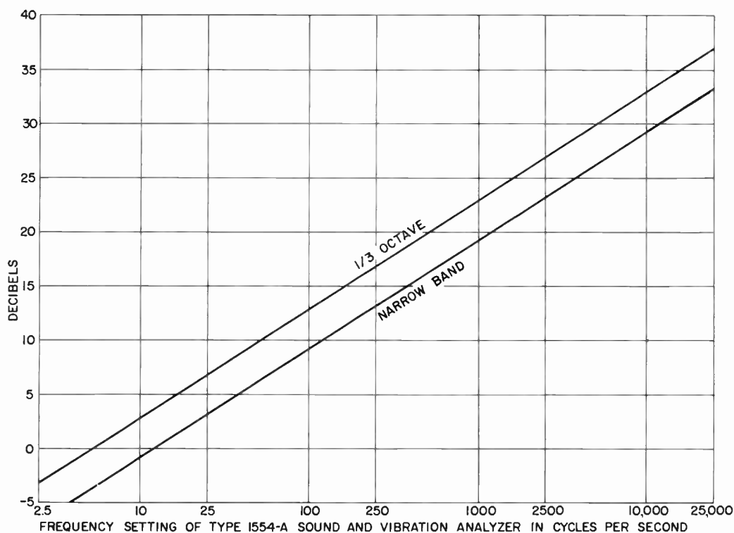
Figure 6-7. Plot showing number of decibels to be subtracted from Type 1554-A readings to obtain spectrum level.
