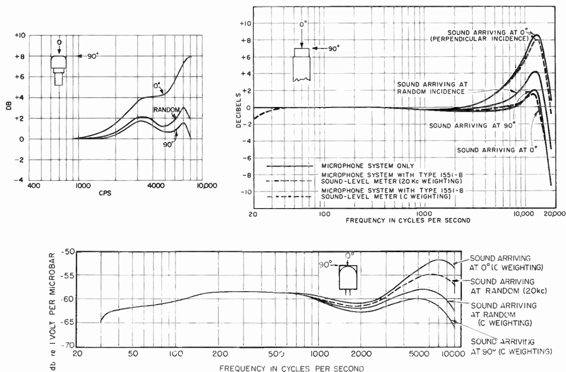
Figure 6-8. Typical response curves for three different microphones when used with the Type 1551-B Sound-Level Meter. (Top left) (a) Rochelle-salt crystal microphone normally supplied with the Type 1551-B; (top right) (c) the Type 1551-P1 Condenser Microphone; (bottom) (b) the Type 759-P25 Dynamic Microphone. Random response assumes that the microphone is placed in a diffuse sound field.
