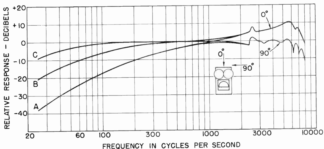
Figure 6-2. Typical over-all free-field response characteristics for the Type 1555-A Sound Survey Meter.
