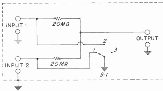
Figure 12-12. A convenient arrangement of a summing circuit for use at the input of the Type 761-A Vibration Meter.
