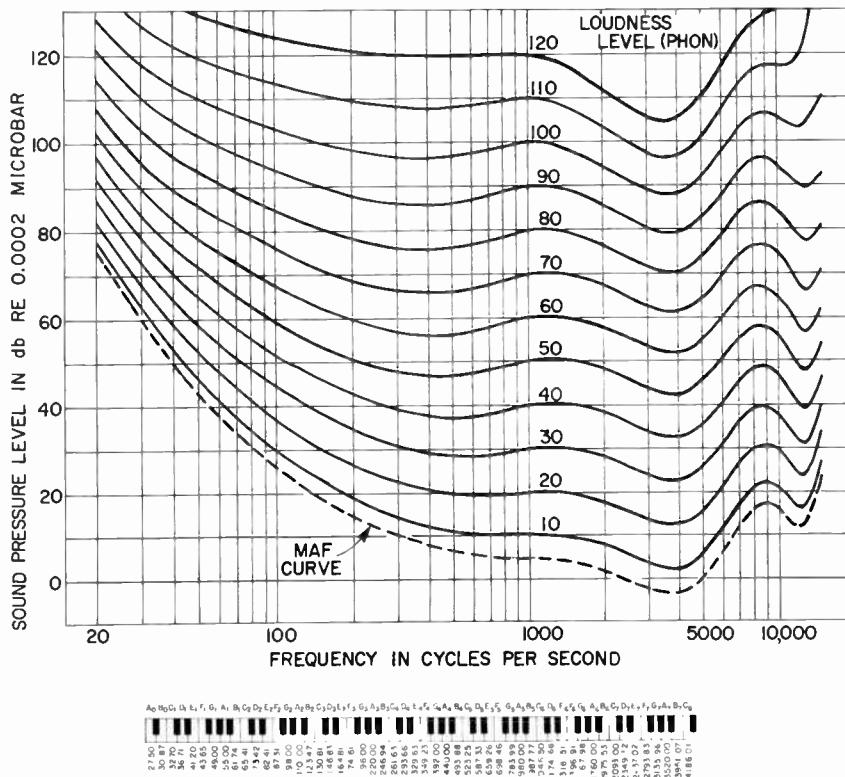
Figure 3-3. Free-field equal-loudness contours for pure tones, determined by Robinson and Daddison at the National Physical Laboratory, Teddington, England. Piano keyboard helps identify the frequency scale. Only the fundamental frequency of each piano key is indicated.
