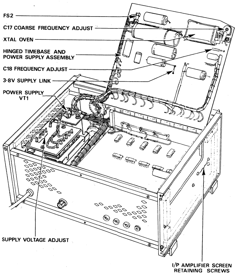
Fig. 6 Component Layout
