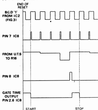
(b) Reclocking Circuit
