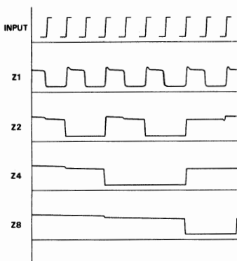
(a) B.C.D Decade Outputs
