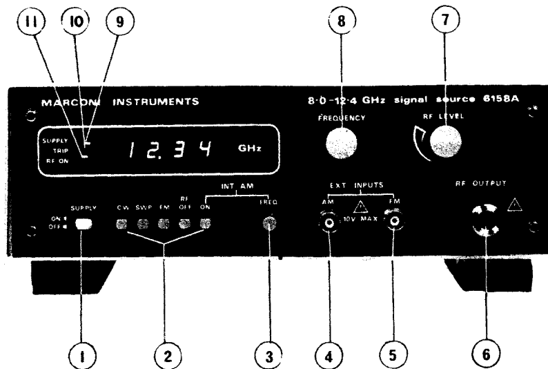
Fig.1 Front Panel
