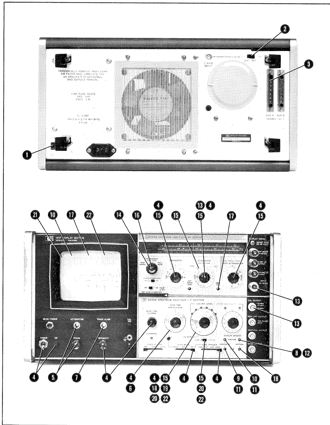
Figure 3-3. Operational Adjustments
