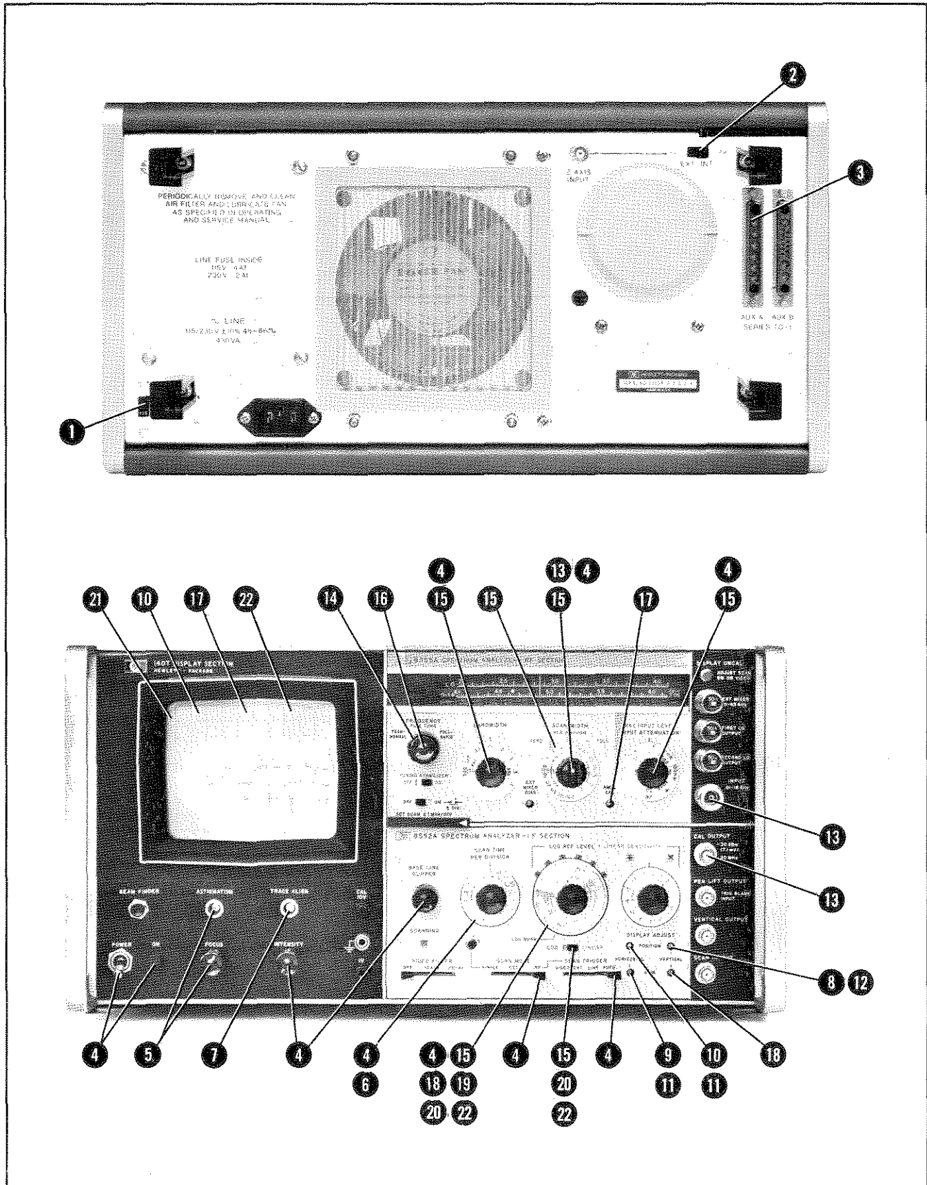
Figure 3-3. Operational Adjustments
