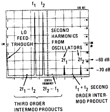
Figure 4-8. Intermodulation Distortion Products Display
