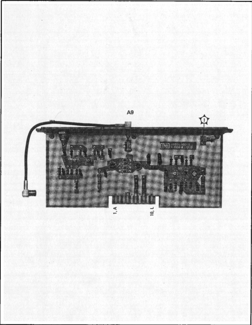
SERVICE SHEET 6 Figure 8-27. Tracking Generator Frequency Converter Assy A9 Component Locations
