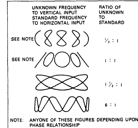
Fig. 34 Lissajous' waveforms used for frequency measurement
