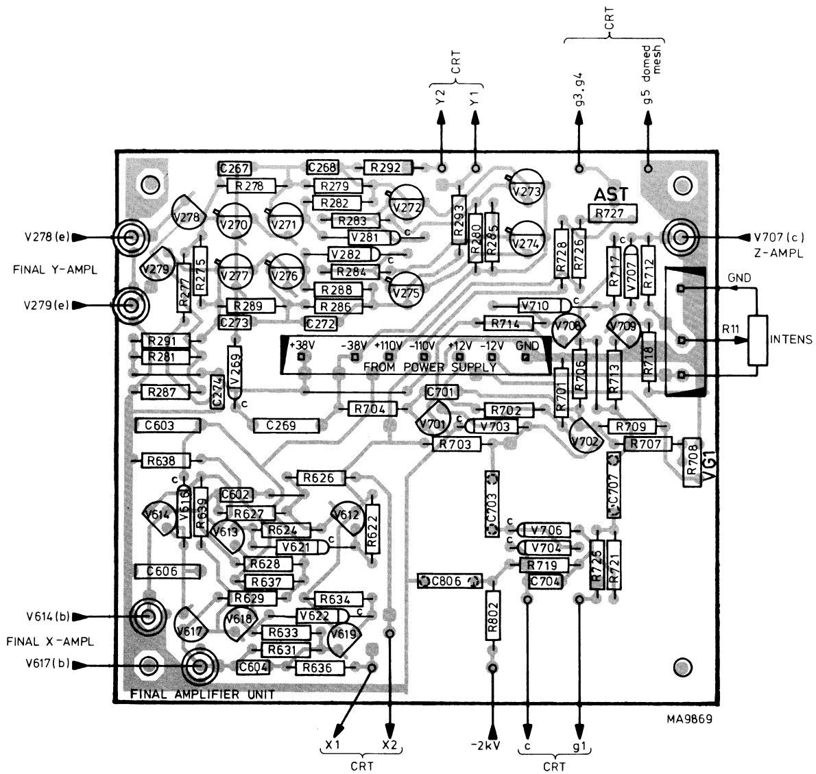
Fig. 3.16. Final amplifier unit, components lay-out
