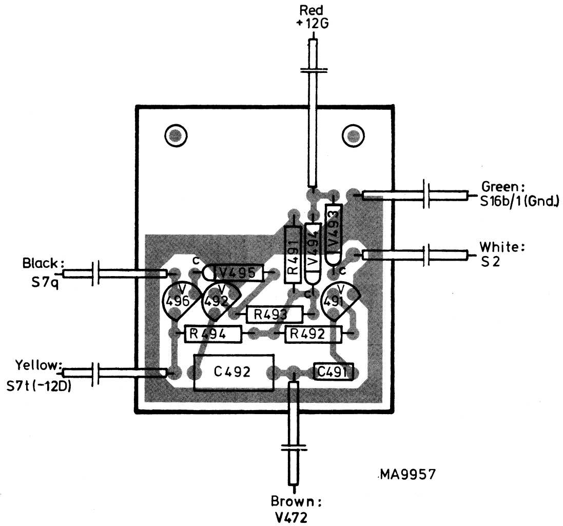
Fig. 3.17. TV trigger unit, components lay-out
