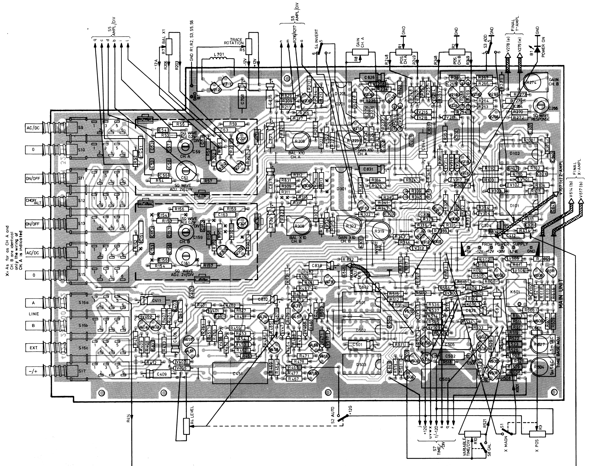
Fig. 3.18. Main unit, components lay-out
