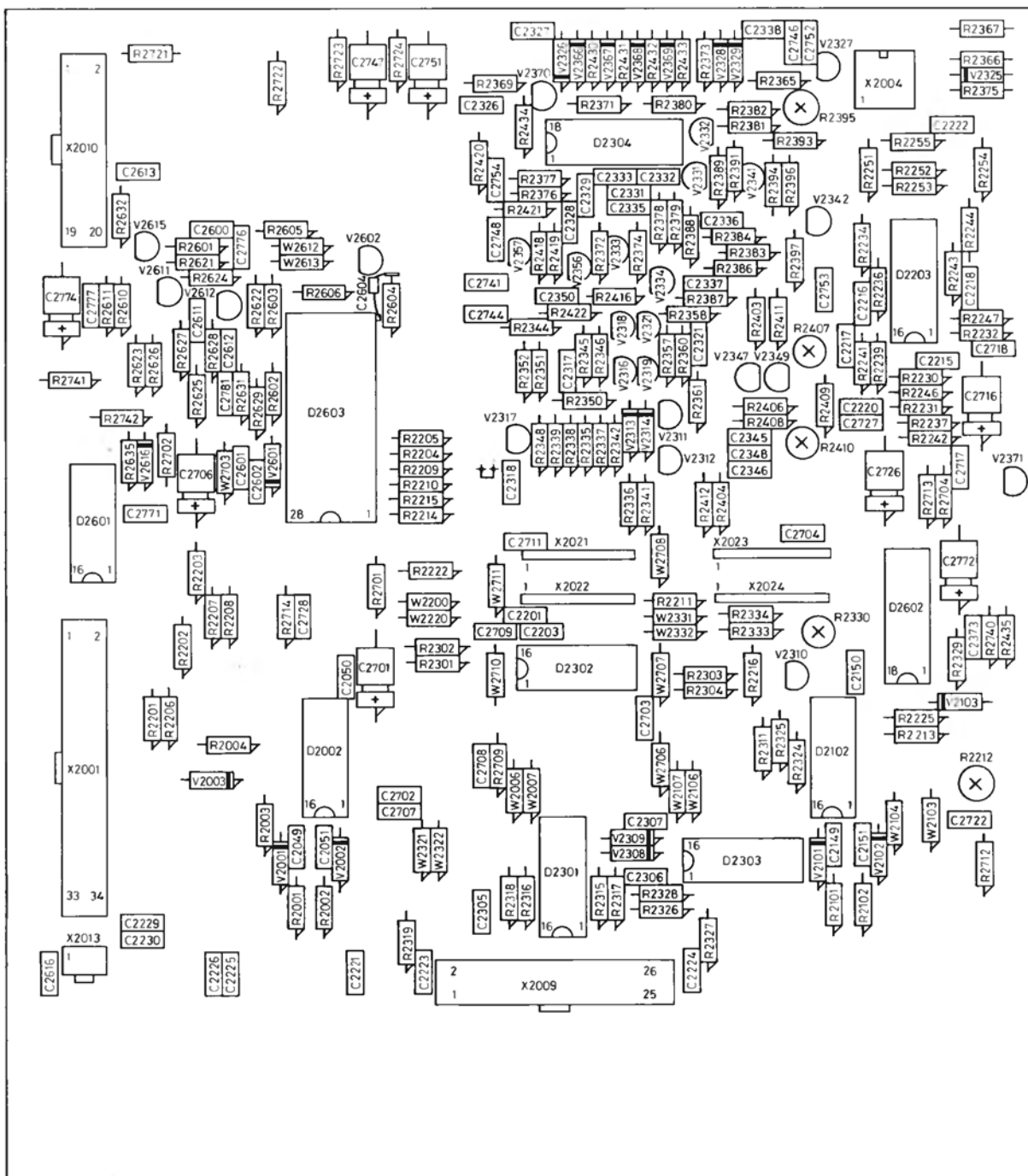
Figure 5.2 Pre-amplifier unit p.c.b.
