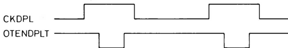
Figure 11.2 Timing diagram of signal transfer
