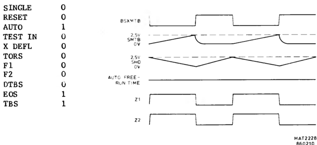
Figure 7.3 Free-running sweep-timing diagram
