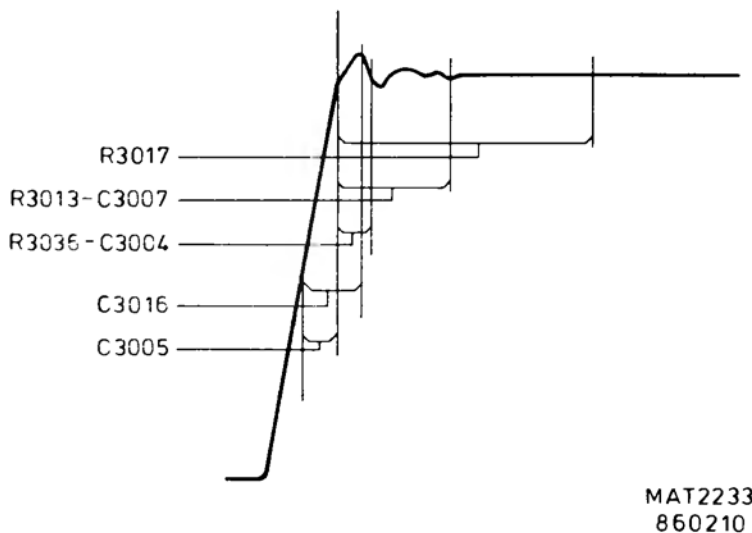
Figure 15.3 Square-wave response
