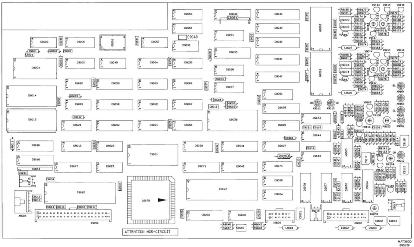
Figure 11.4 Digital unit, p.c.b. lay-out
