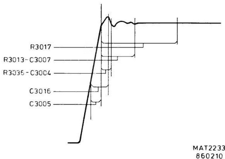
Figure 15.3 Square-wave response
