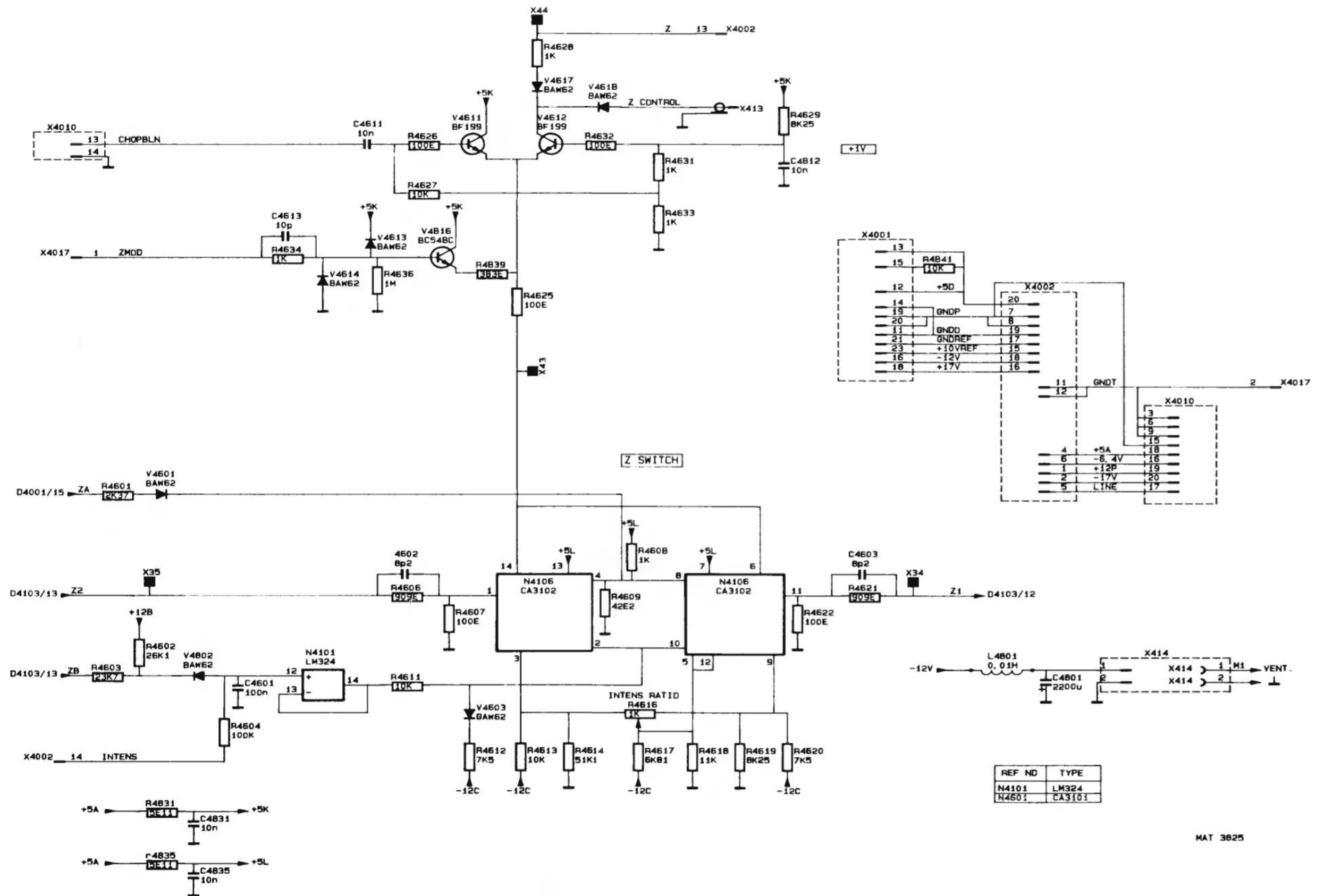
Figure 7.10 Circuit diagram of time-base, Z-amplifier
