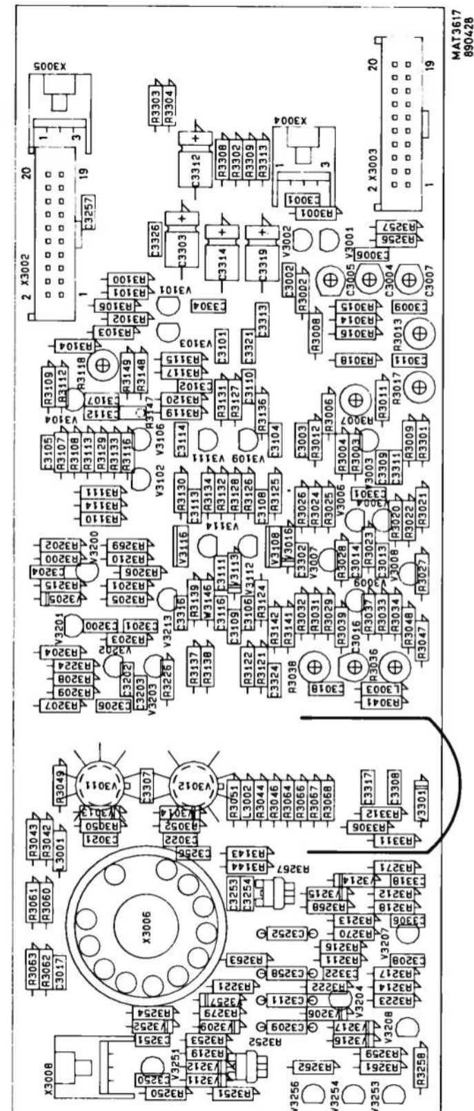
Figure 6.1 XYZ amplifier p.c.b.
