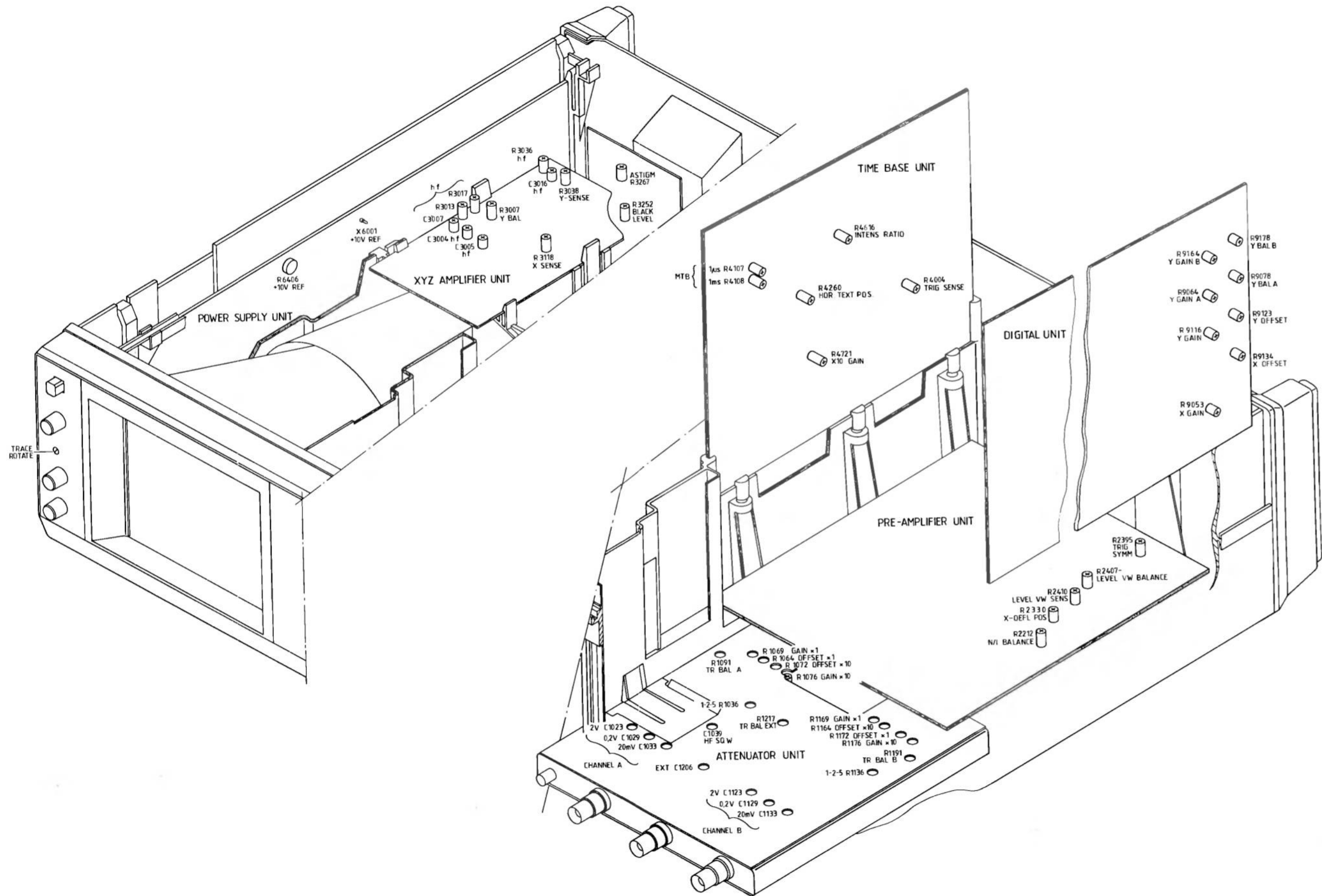
Figure 15.1 Adjusting elements
