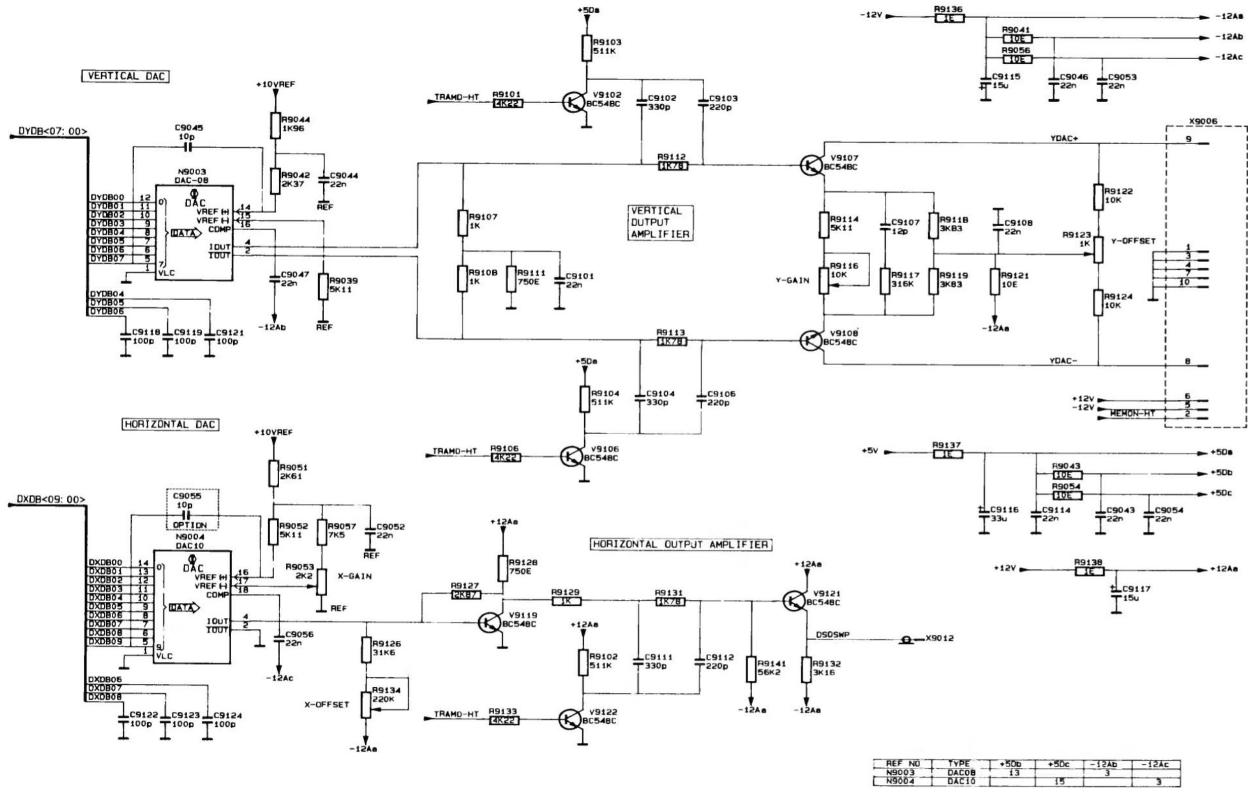
Figure 11.9 Circuit diagram of DAC-circuits
