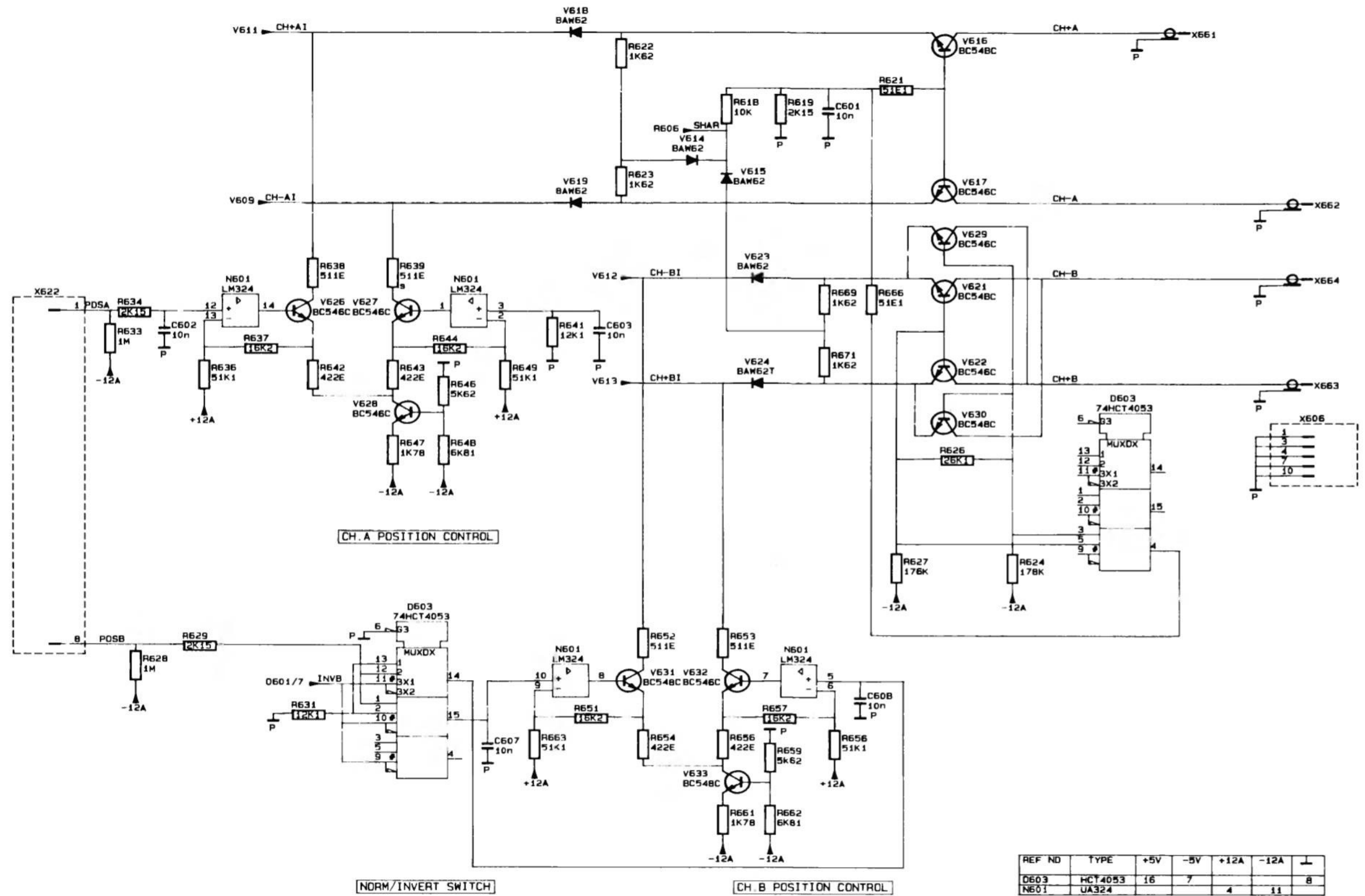
Figure 12.3 Circuit diagram of adaptation unit, section 2
