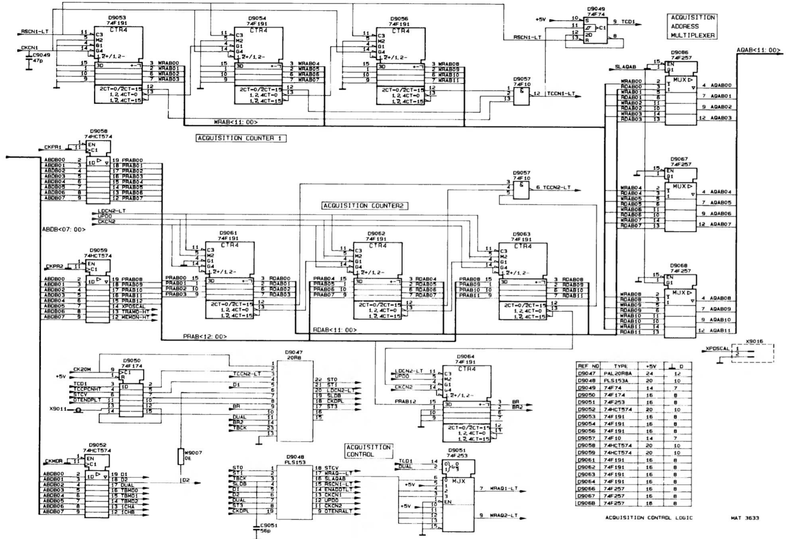
Figure 11.7 Circuit diagram of aquisition control logic
