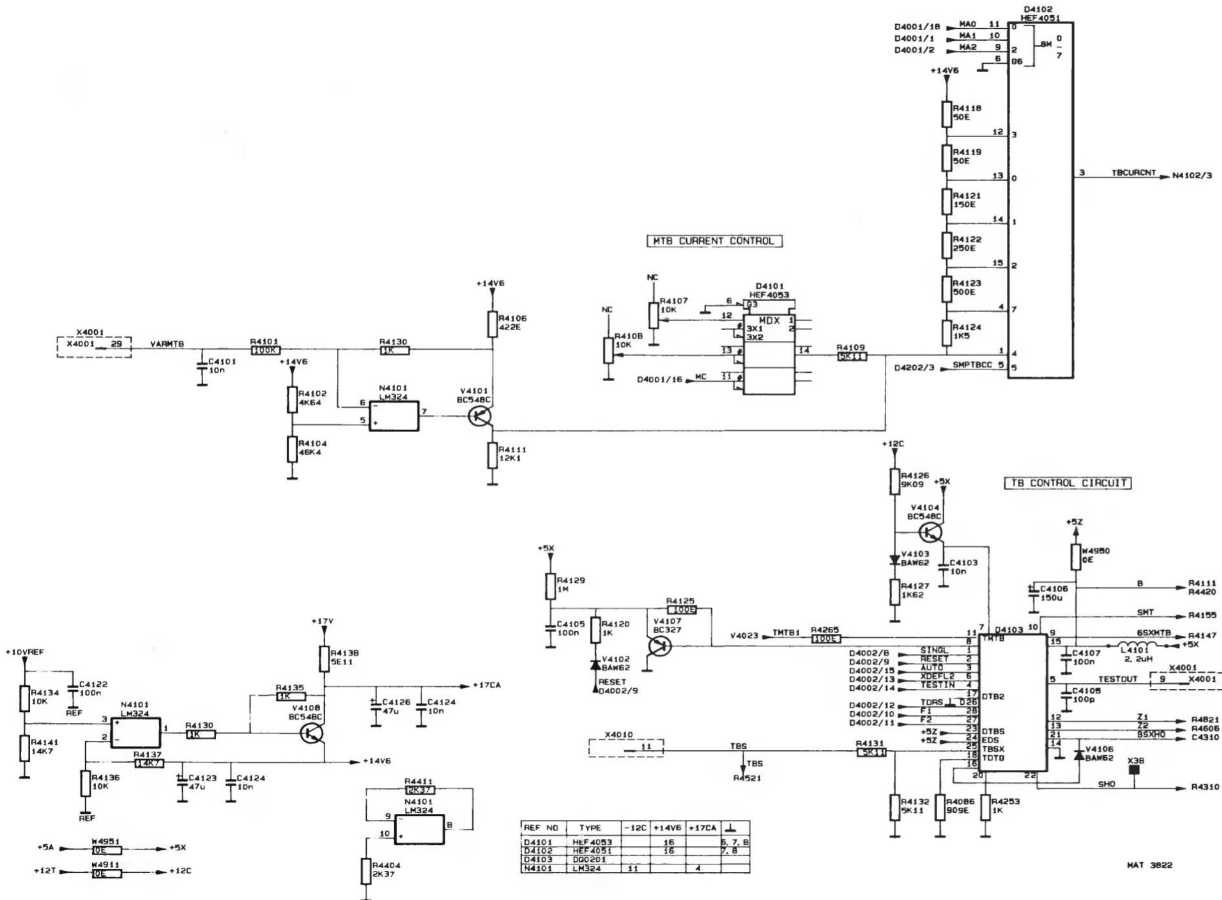
Figure 7.6 Circuit diagram of time-base, timing circuit and control
