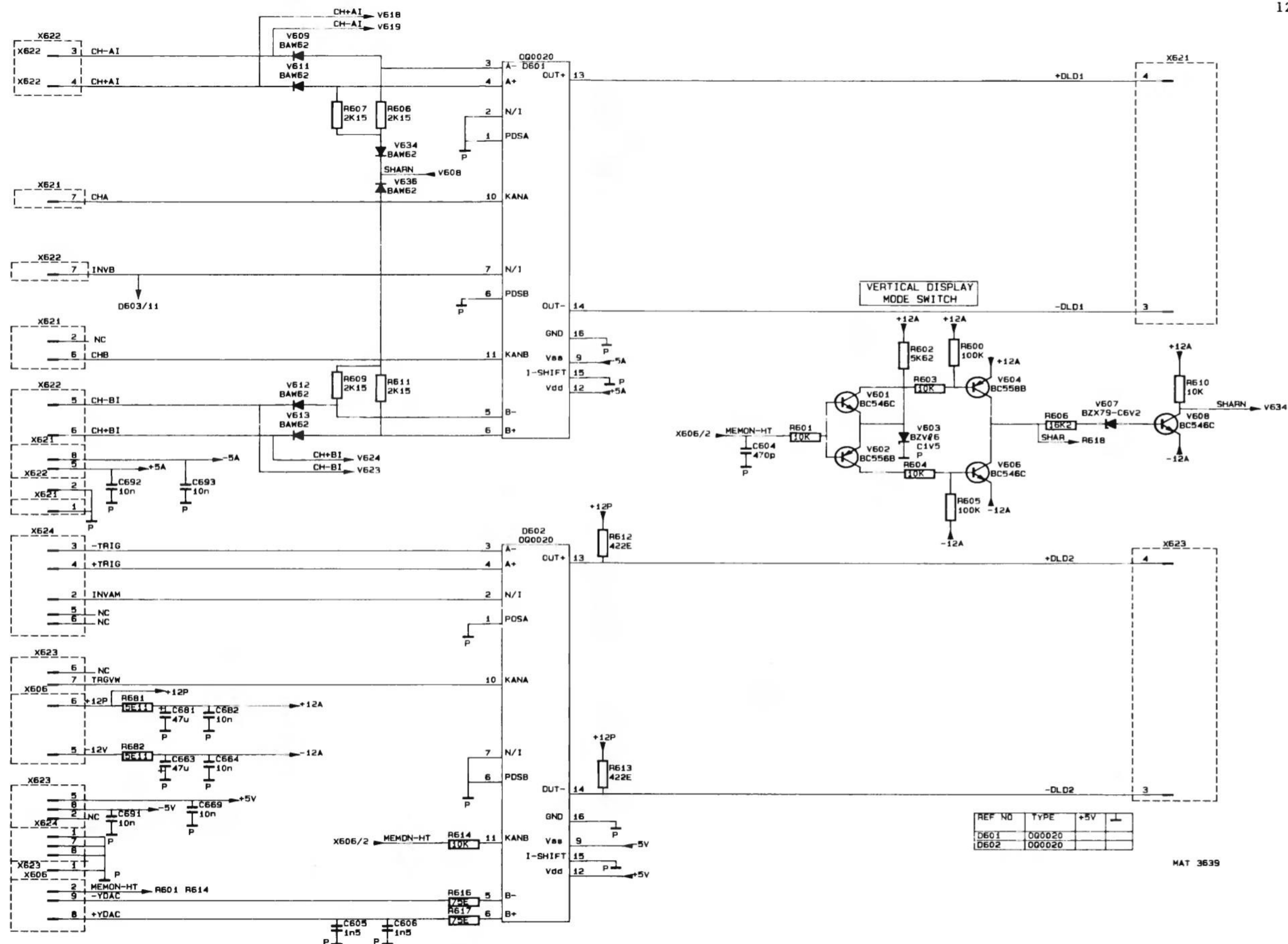
Figure 12.2 Circuit diagram of adaptation unit, section 1
