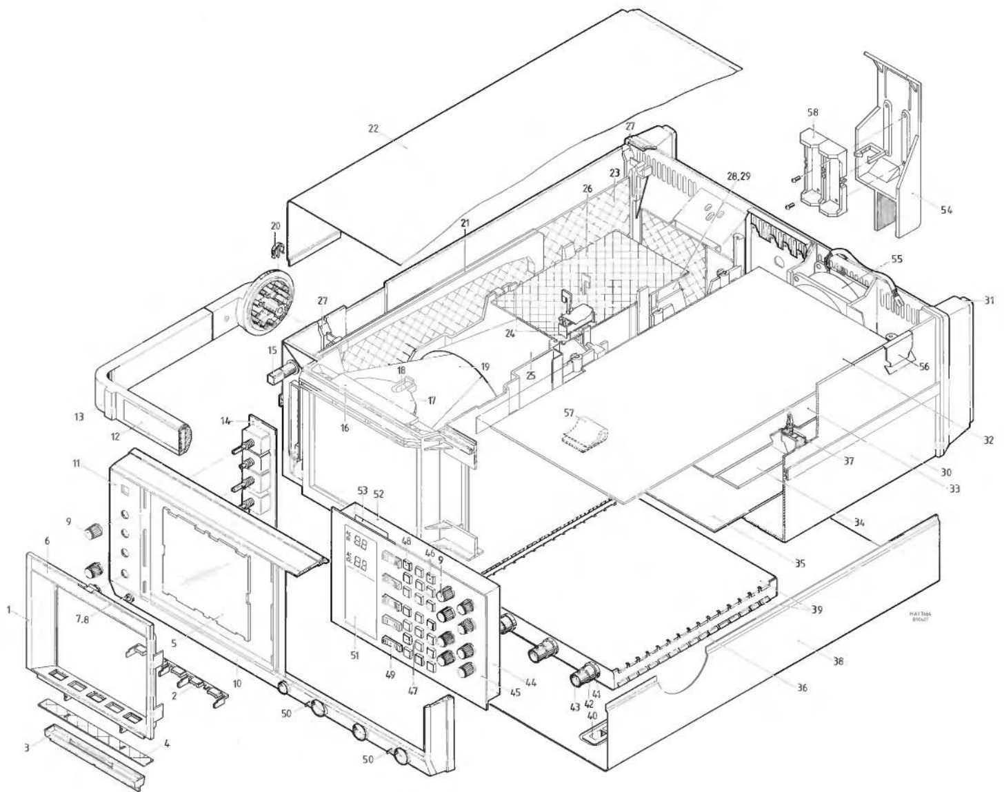
Figure 18.1 Exploded view
