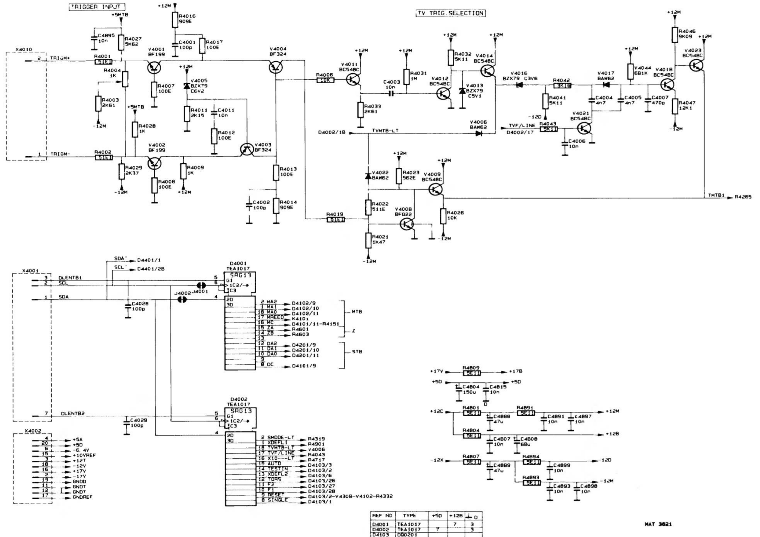
Figure 7.5 Circuit diagram of time-base, trigger amplifier
