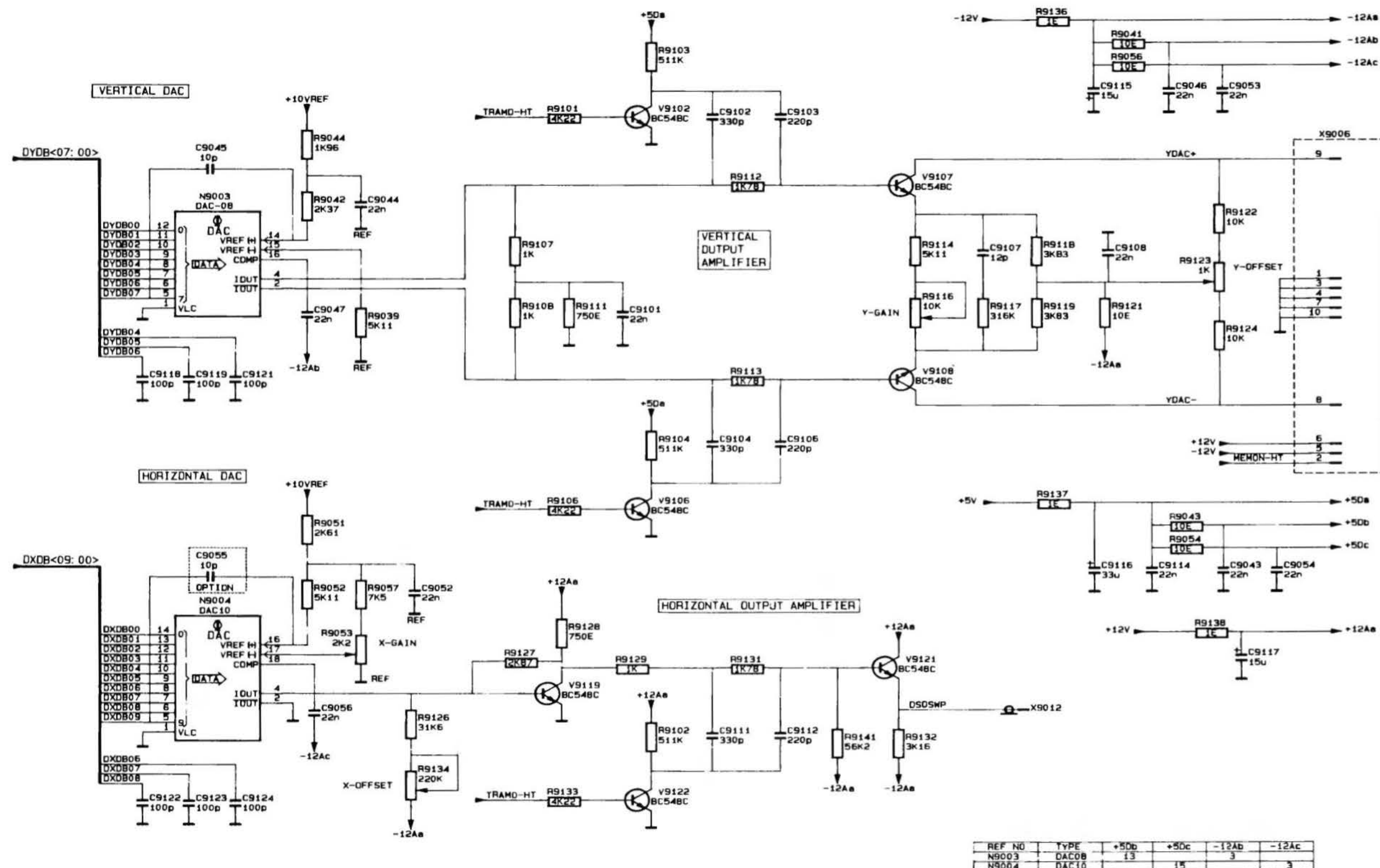
DAC CIRCUITS MAT 3835
