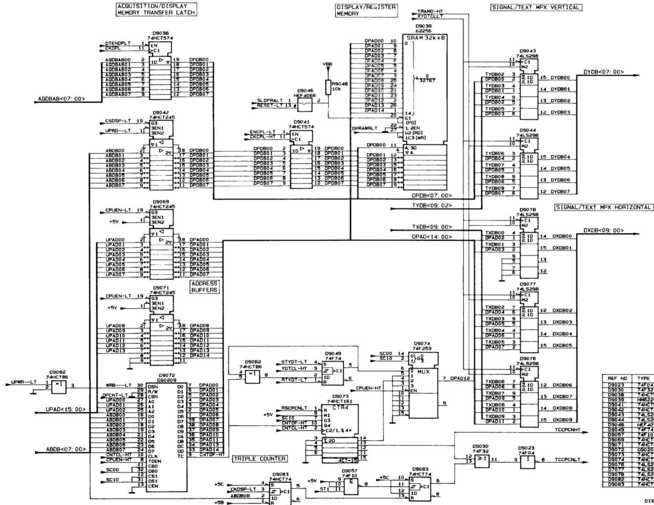
Figure 11.8 Circuit diagram of display logic
