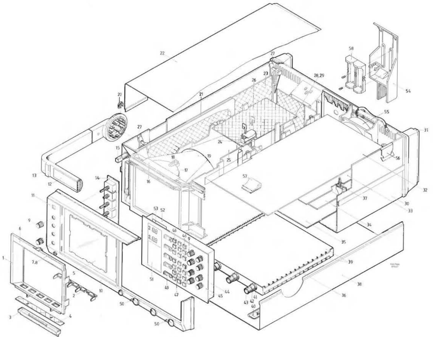
Figure 18.1 Exploded view
