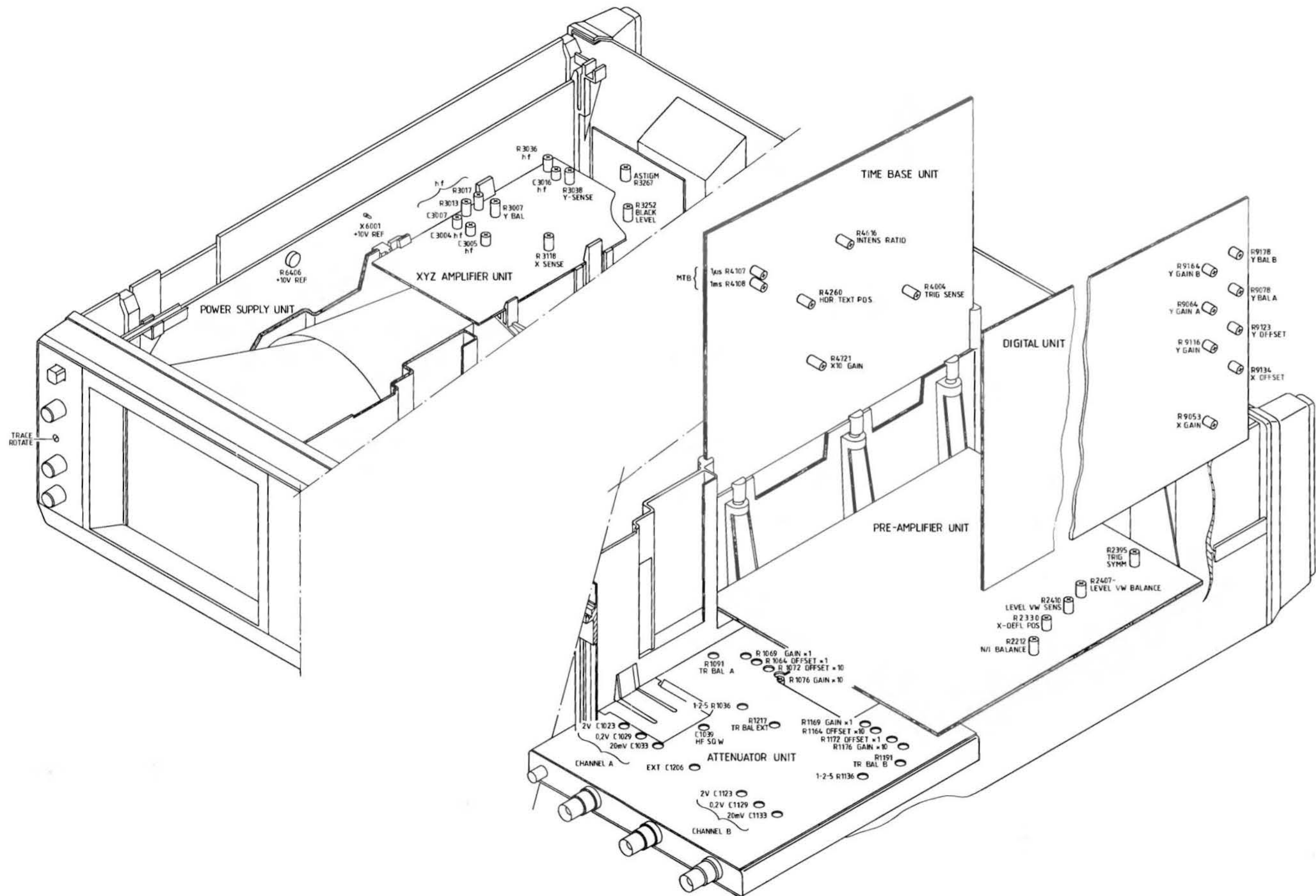
Figure 15.1 Adjusting elements
