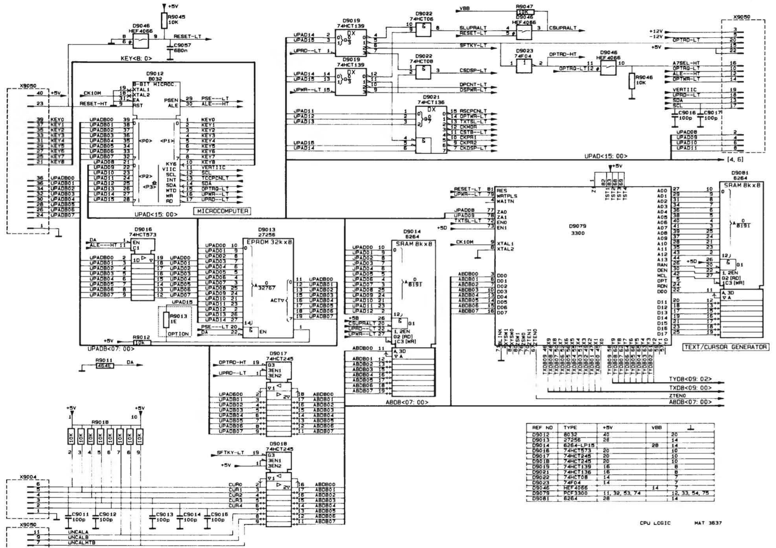
Figure 11.11 Circuit diagram of CPU logic
