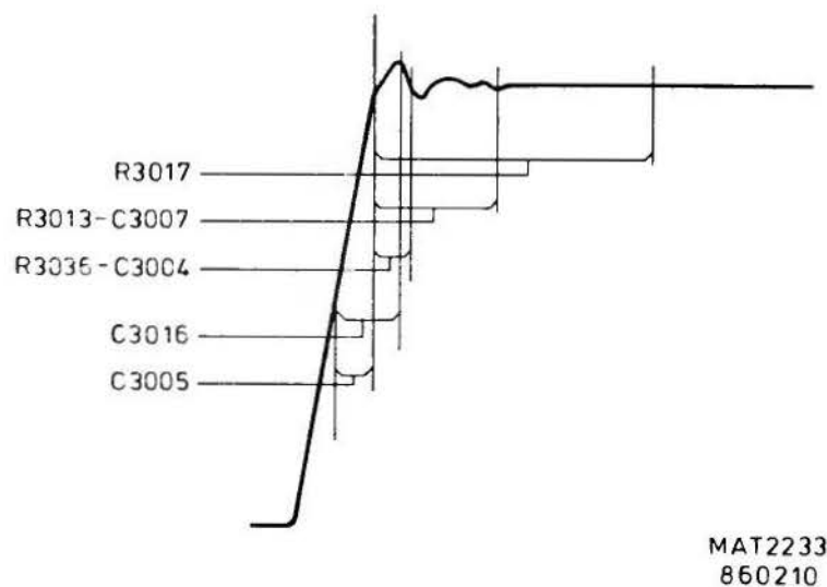
Figure 15.3 Square-wave response
