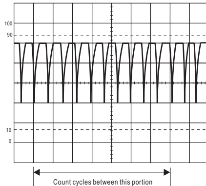
Fig. 10 Alternate Method Of Frequency Measurement
