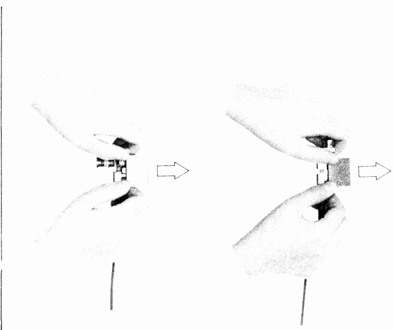
Figure 9. Removing matching-box cover _____
