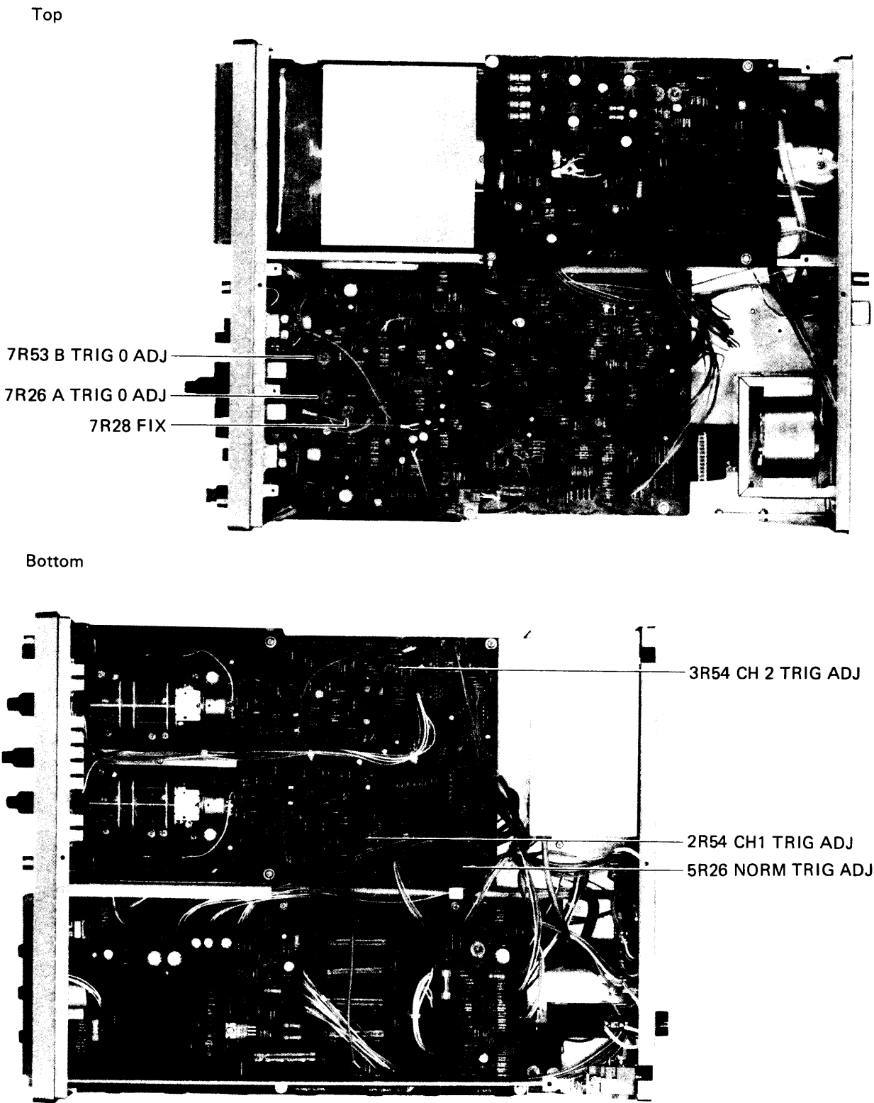
Figure 6-10-1. Location of calibrators (Trigger system)
