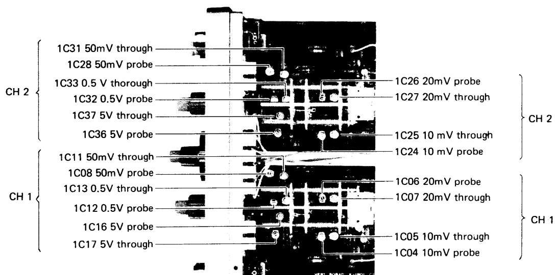
Figure 6-9-1. Adjustment location (Attenuator compensation)
