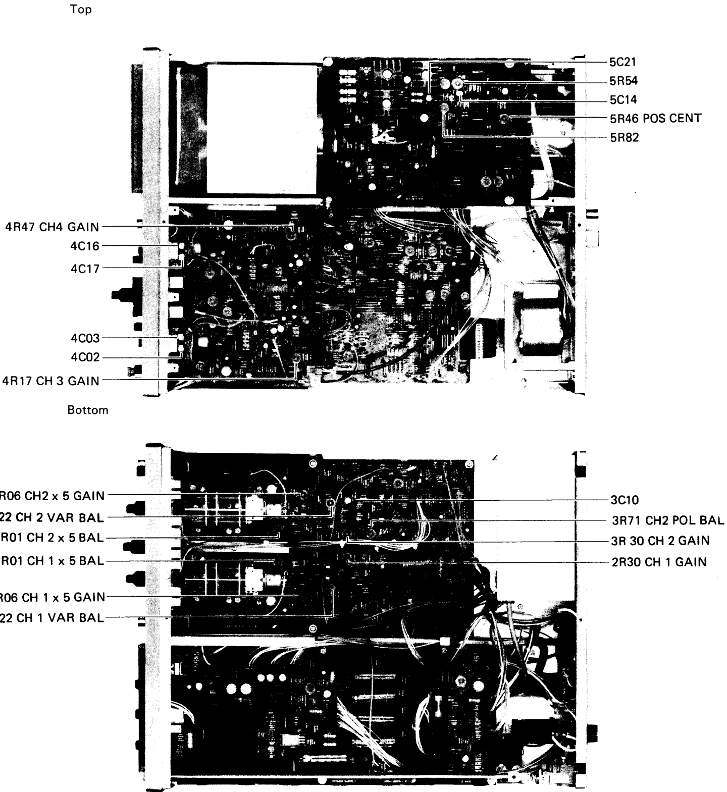
Figure 6-9-1. Location of calibrators (Vertical deflection system)
