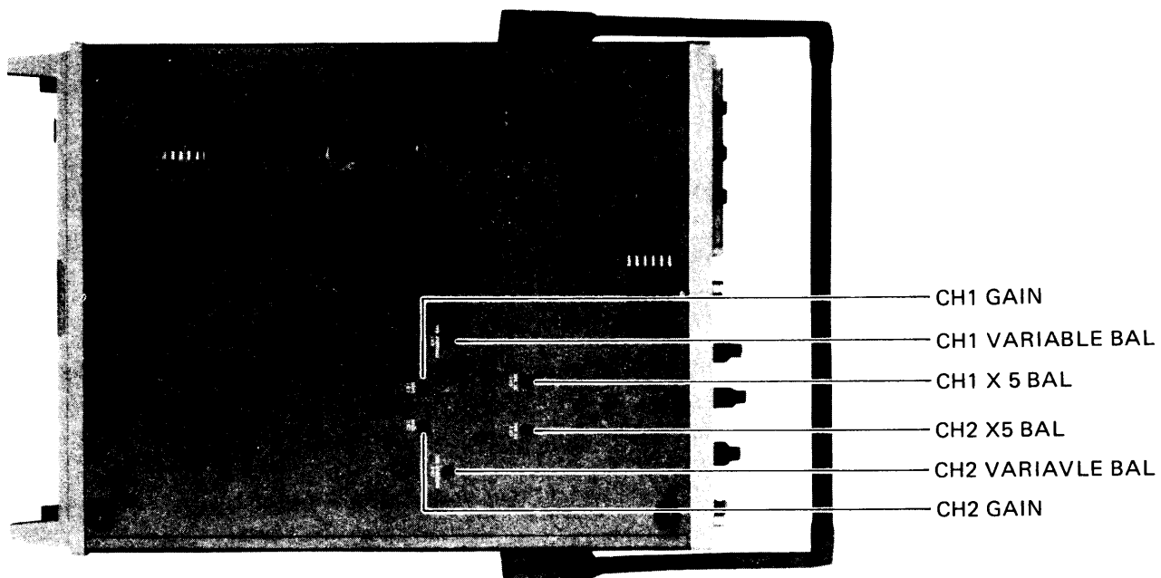
Figure 2-5. Bottom cover
