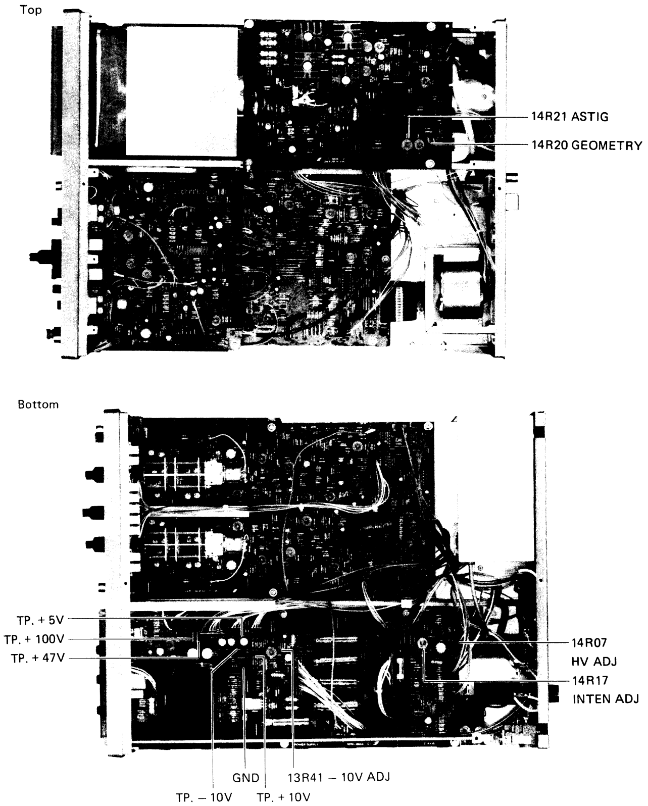
Figure 6-7-2. Adjustment and Testpoint Locations (POWER SUPPLY and CRT)
