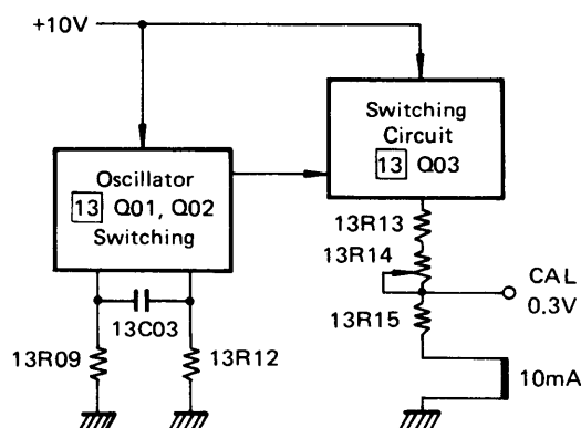
Figure 4-1-16. Block diagram of calibrator
