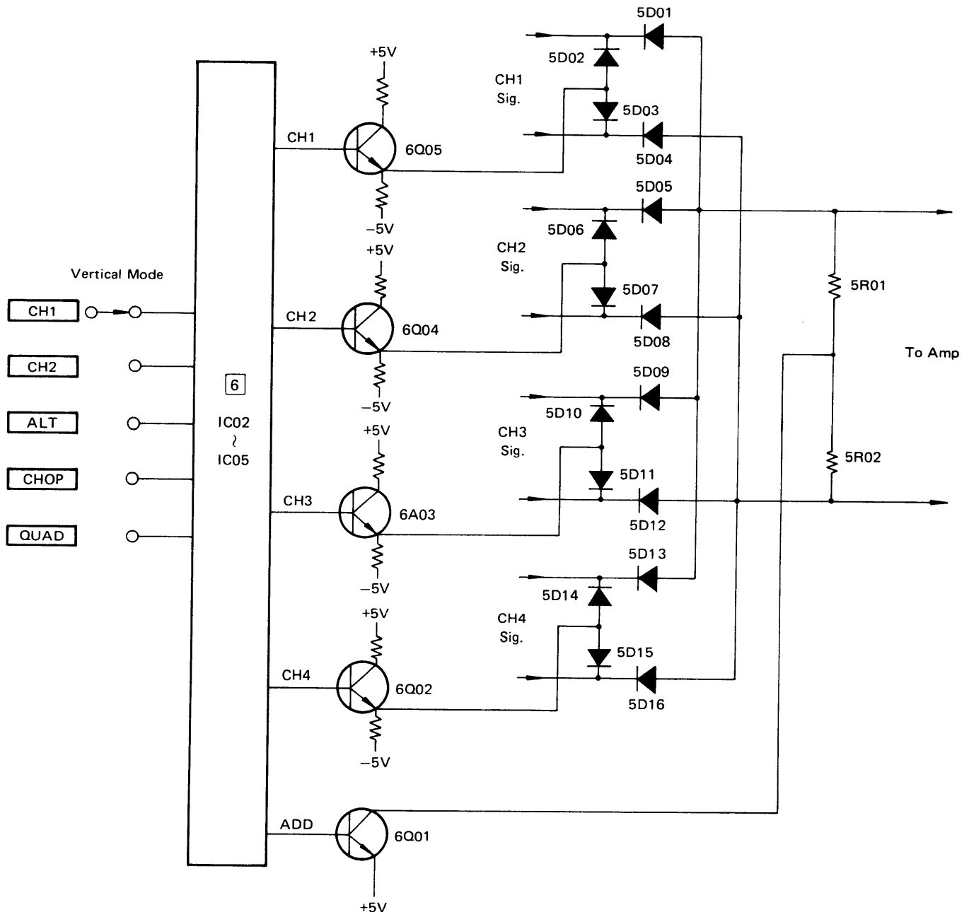
Figure 4-1-5. Switching circuit
