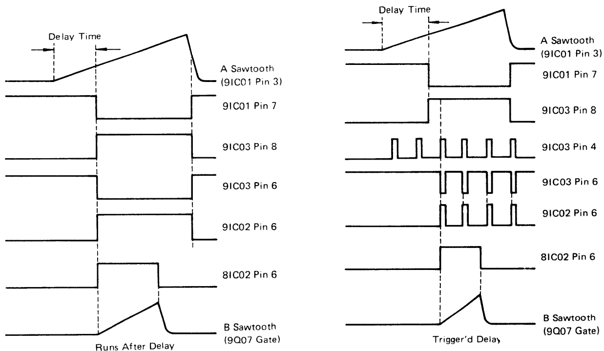
Figure 4-1-12. Timing chart
