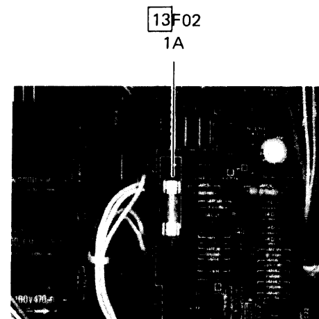
Figure 2-1. Fuse Locations
