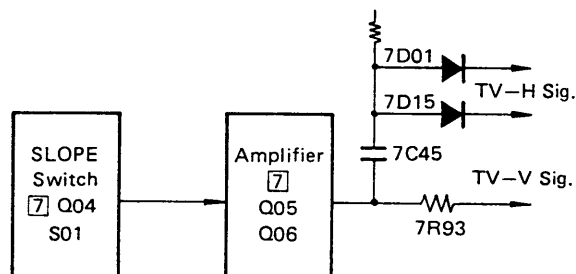
Figure 4-1-7. Block diagram of TV Trigger signal separator
