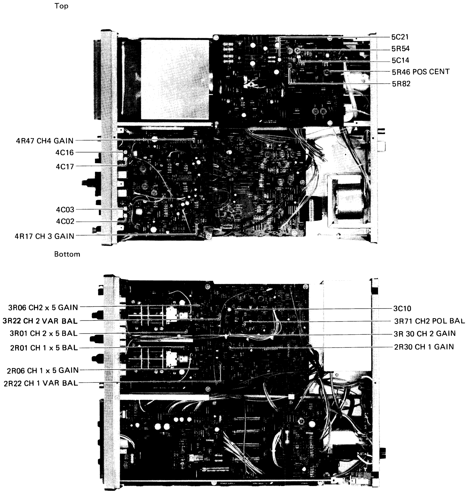
Figure 6-9-1. Location of calibrators (Vertical deflection system)
