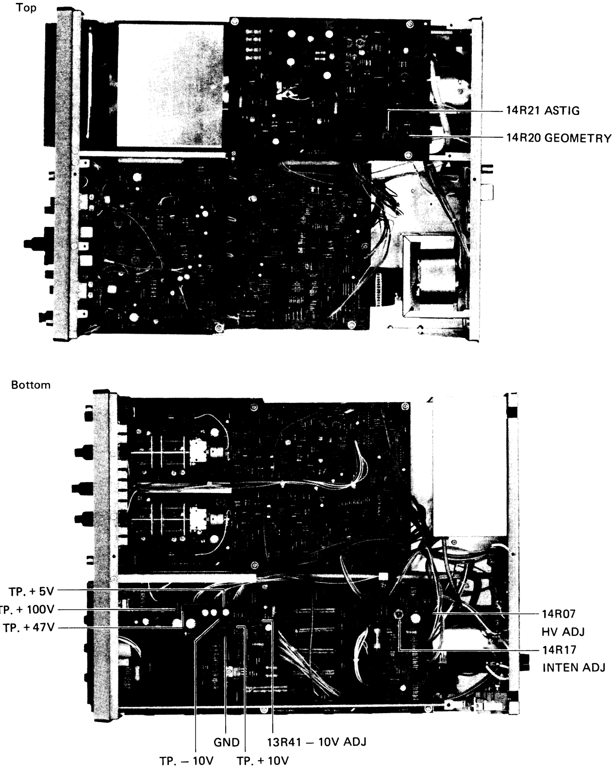
Figure 6-7-2. Adjustment and Testpoint Locations (POWER SUPPLY and CRT)
