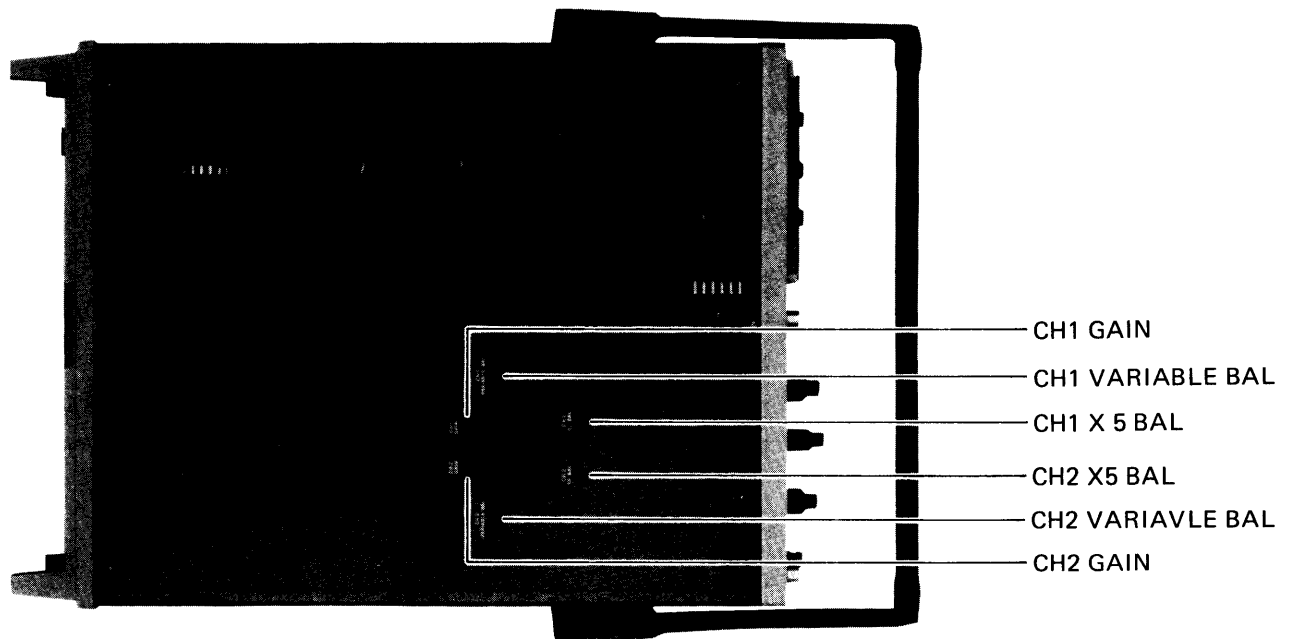
Figure 2-7. Bottom cover
