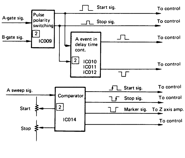
Figure 4-2-4. Block diagram of time interval control
