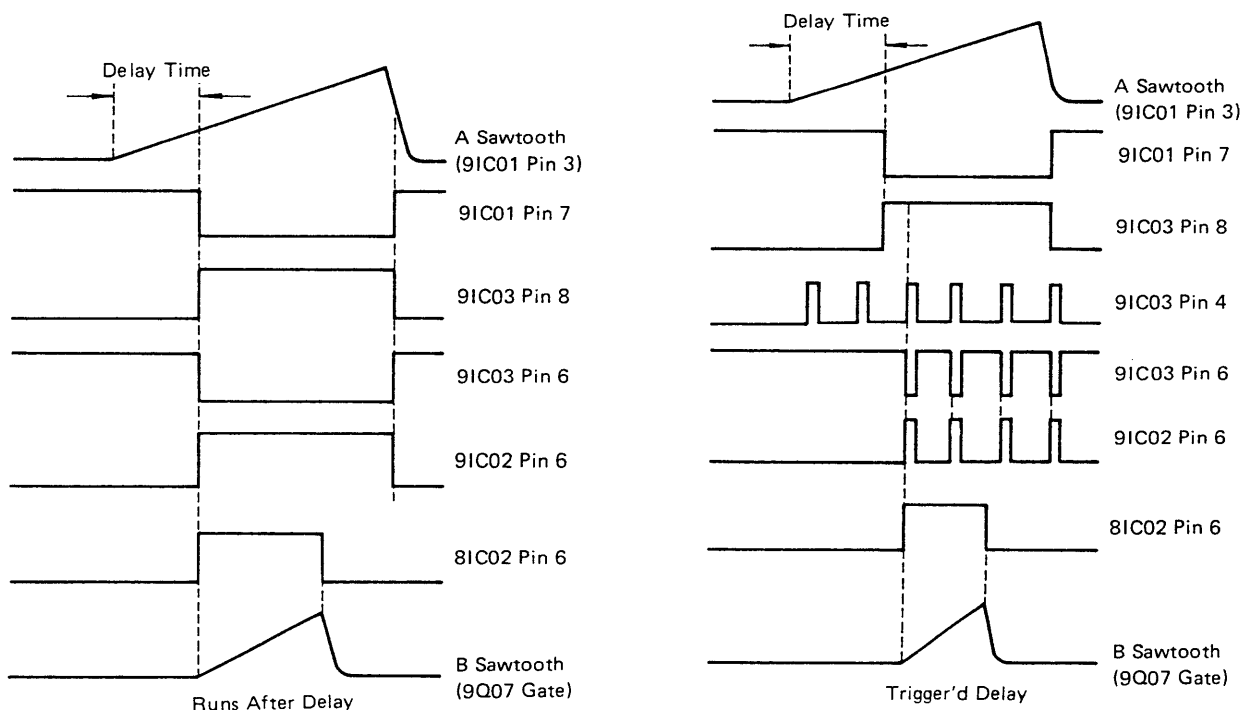
Figure 4-1-12. Timing chart
