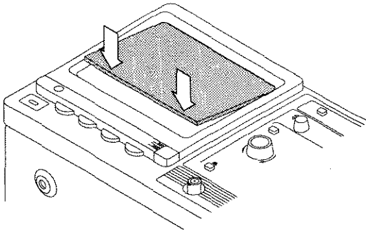
Figure 14: Bezel Replacement (Step 6)
