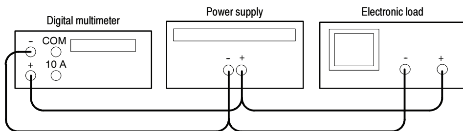
Figure 8: Constant voltage source test setup
