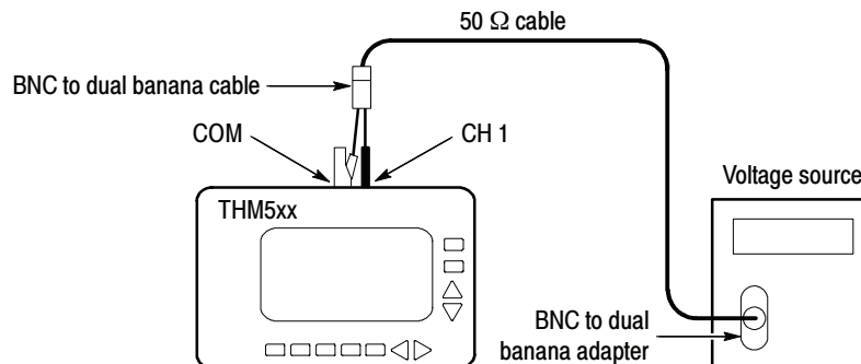
Figure 7: Vertical accuracy test setup
