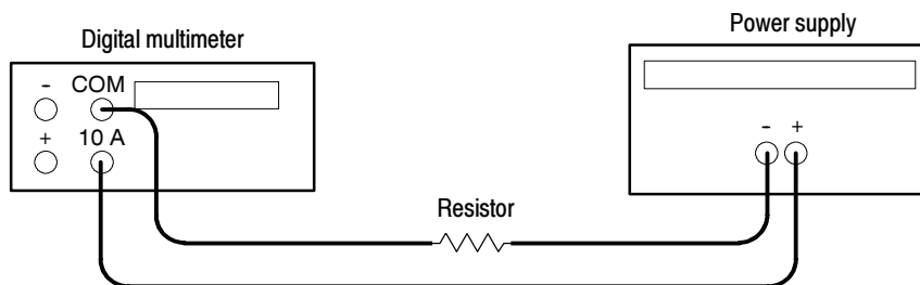
Figure 6: Constant current source test setup
