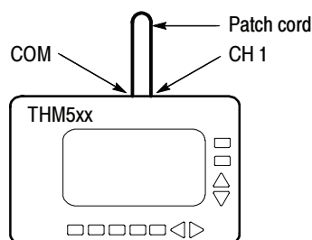
Figure 5: Trace shift test setup
